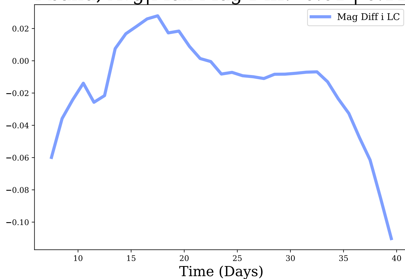
i-band, Avg|Max Mag Diff: -0.01 | 0.11
