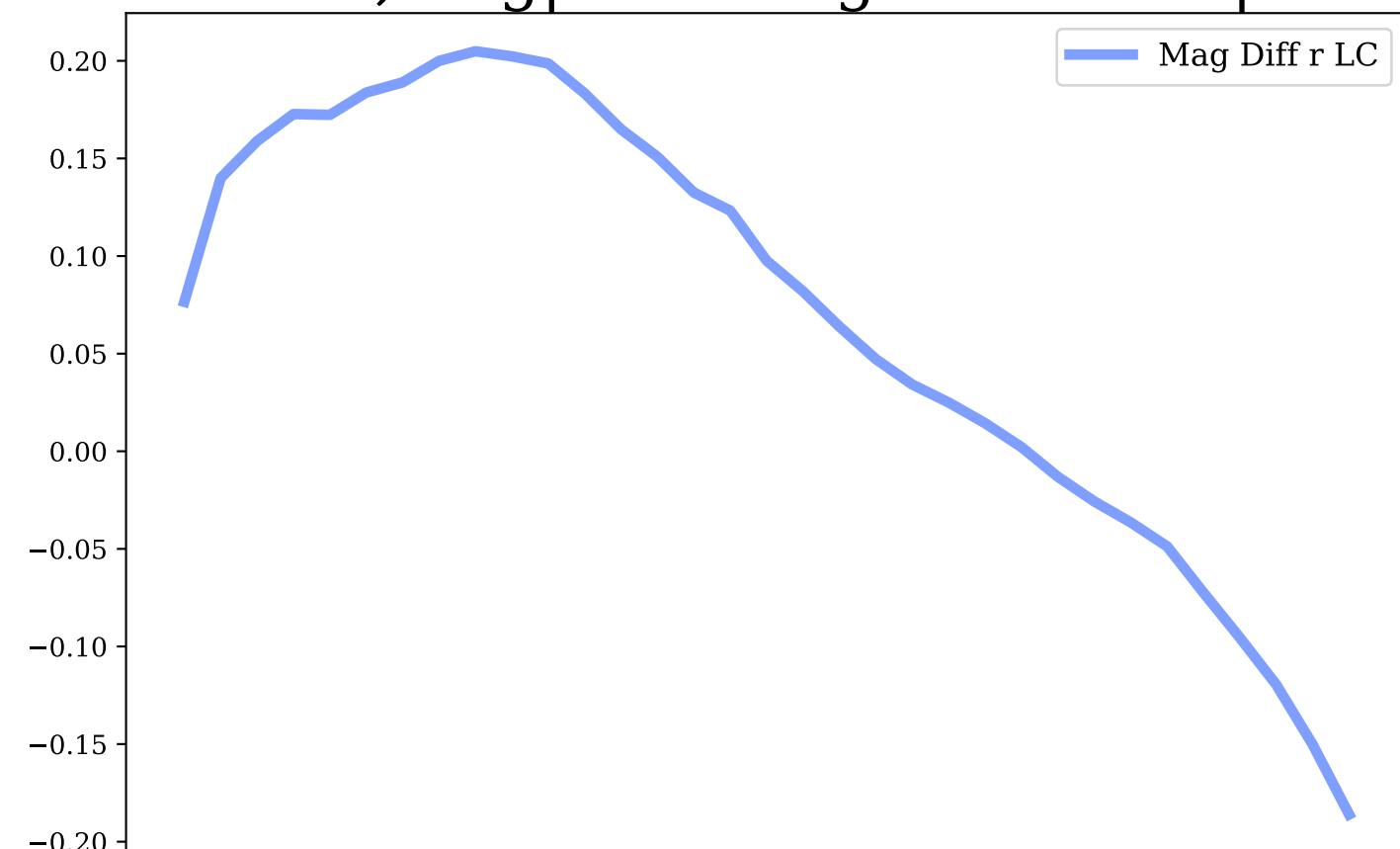
z-band, Avg|Max Mag Diff: -0.06 | 0.13
