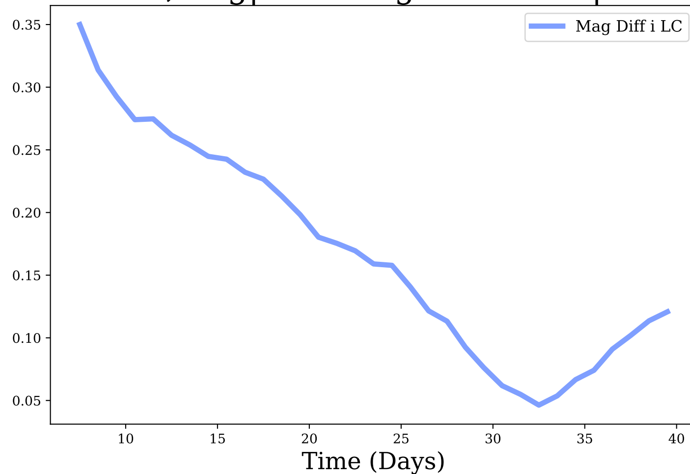
i-band, Avg|Max Mag Diff: 0.17 | 0.35
