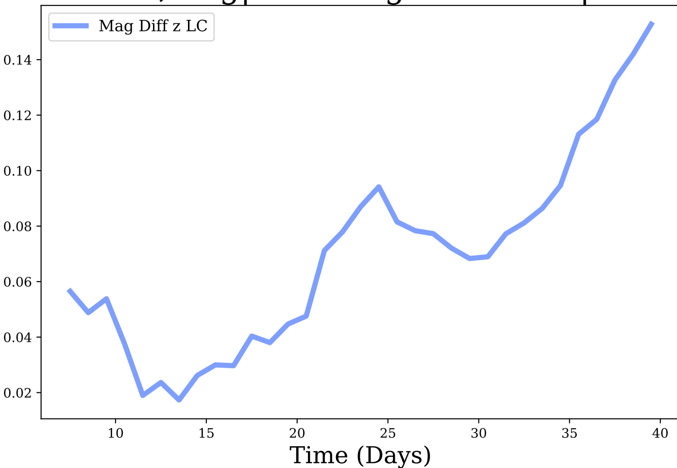
z-band, Avg|Max Mag Diff: 0.07 | 0.15
