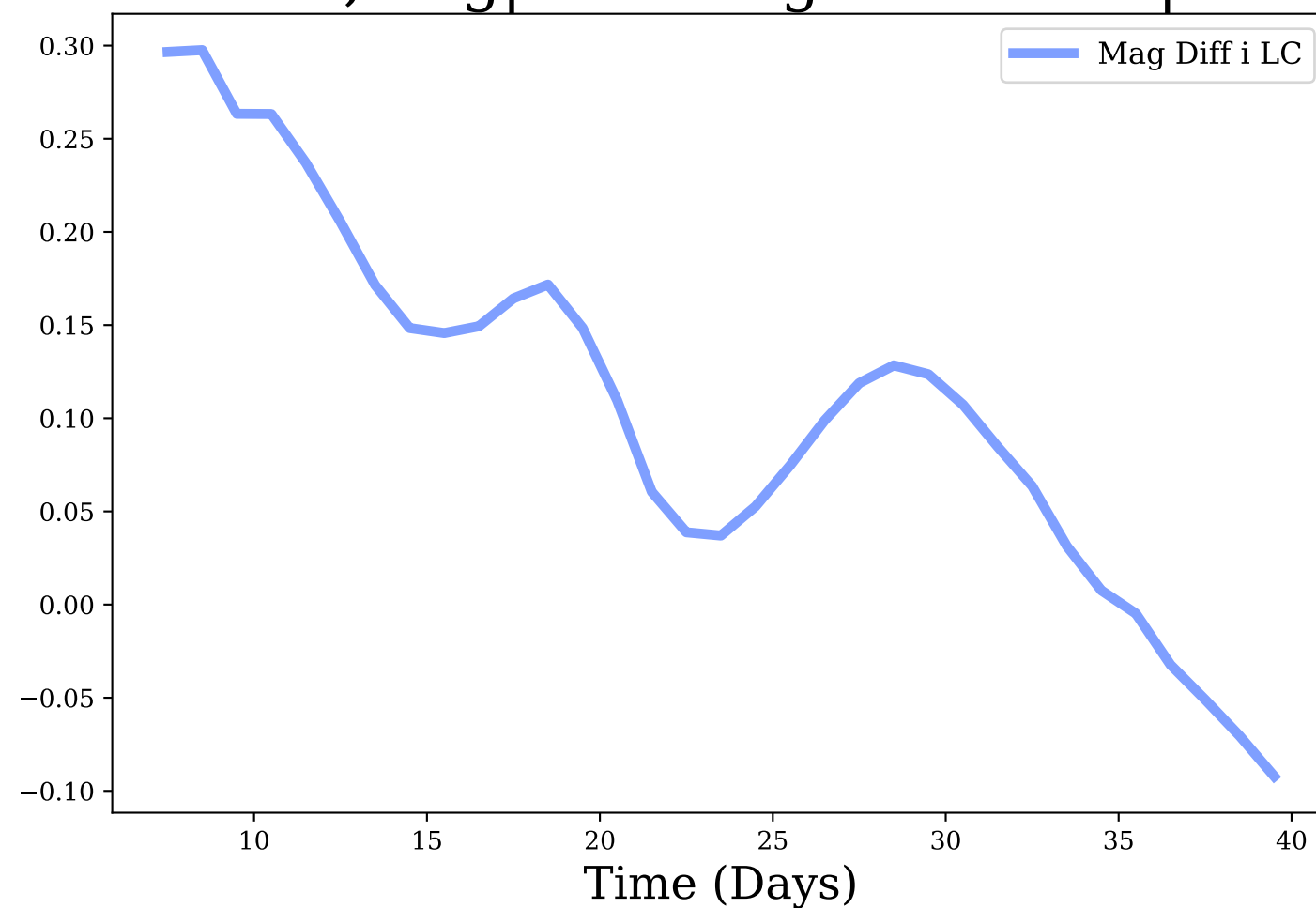
i-band, Avg|Max Mag Diff: 0.11 | 0.3
