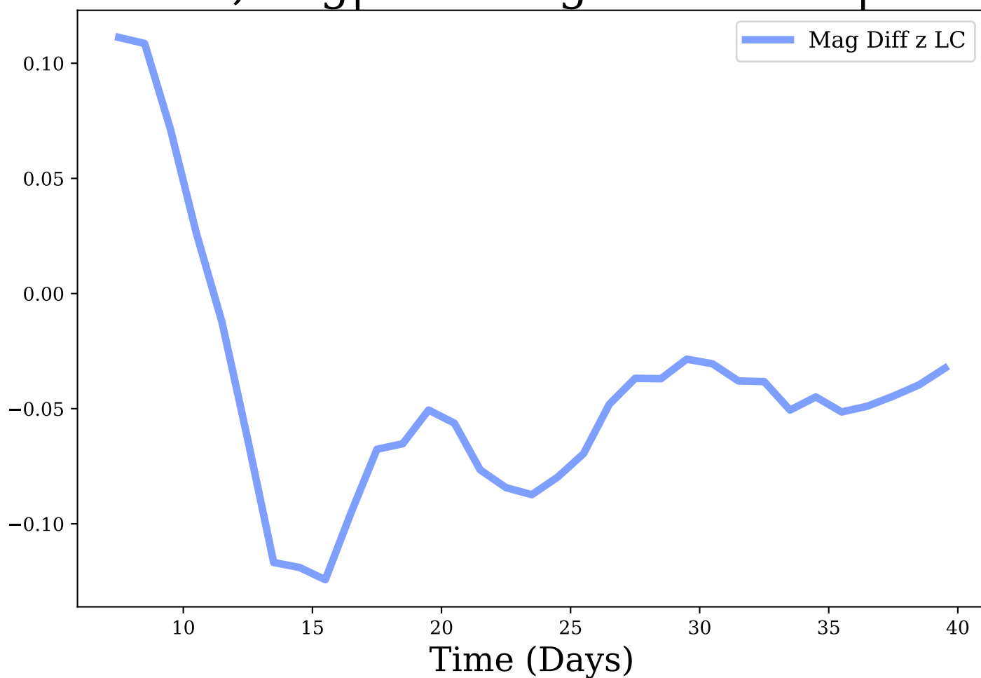
z-band, Avg|Max Mag Diff: -0.04 | 0.12
