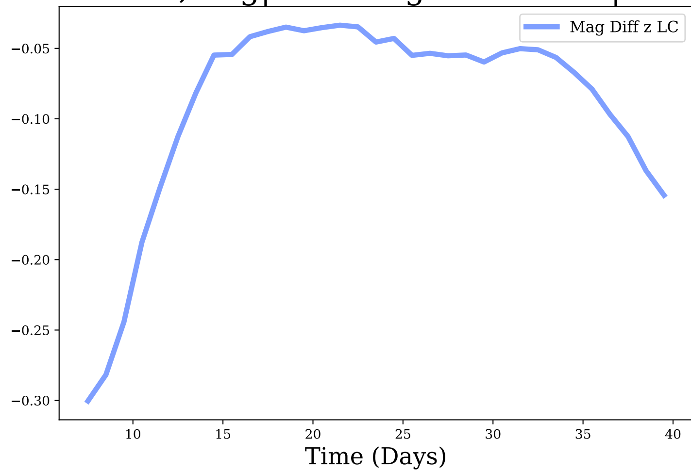
z-band, Avg|Max Mag Diff: -0.09 | 0.3
