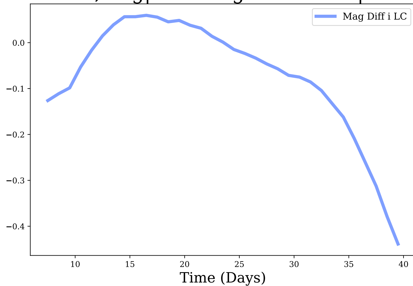
i-band, Avg|Max Mag Diff: -0.07 | 0.44
