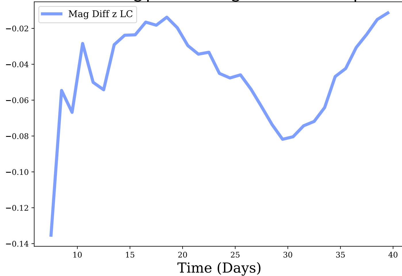
z-band, Avg|Max Mag Diff: -0.05 | 0.14
