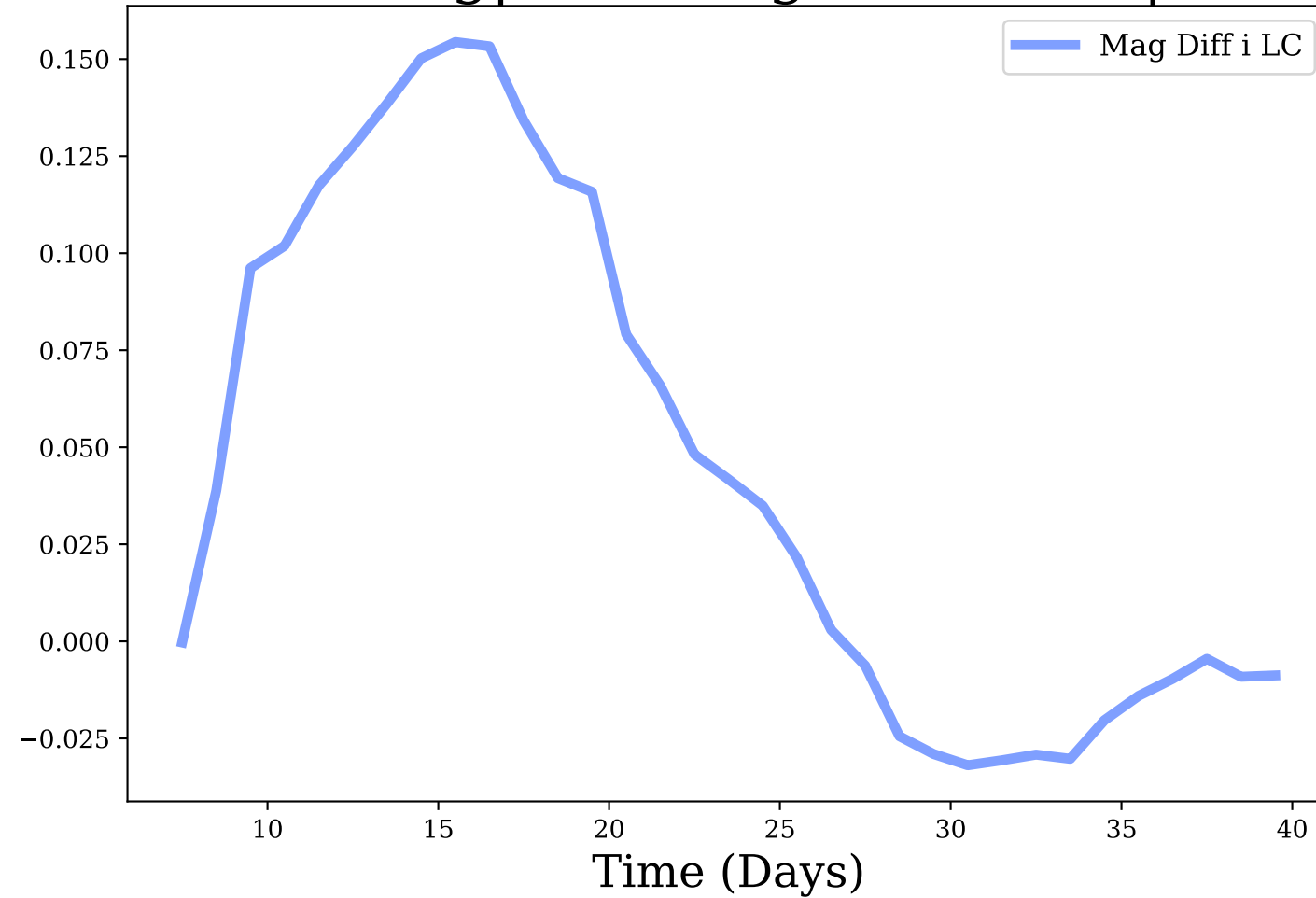
i-band, Avg|Max Mag Diff: 0.05 | 0.15
