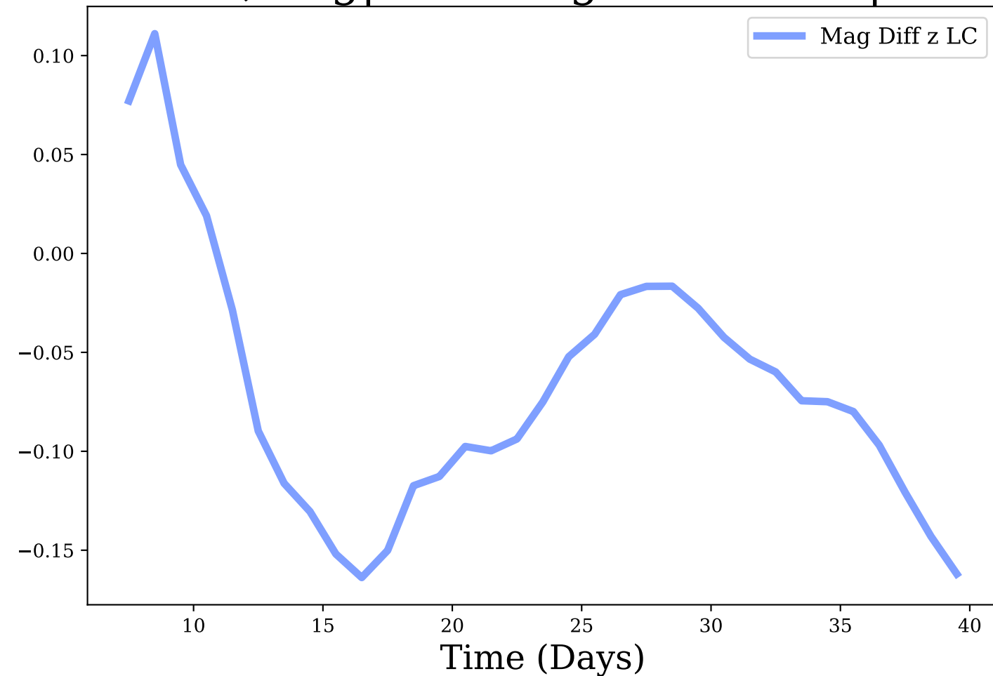
z-band, Avg|Max Mag Diff: -0.07 | 0.16
