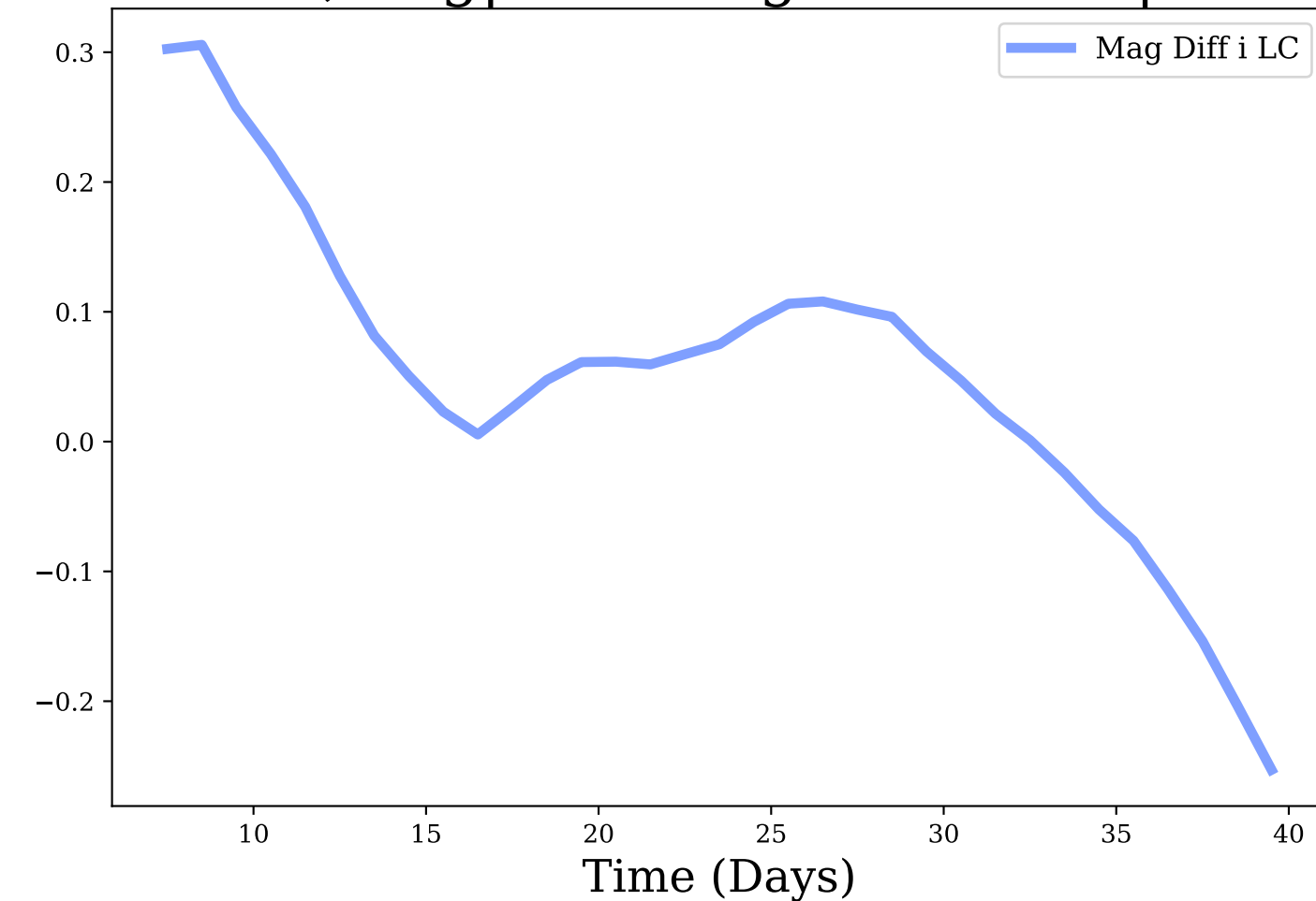
i-band, Avg|Max Mag Diff: 0.05 | 0.31
