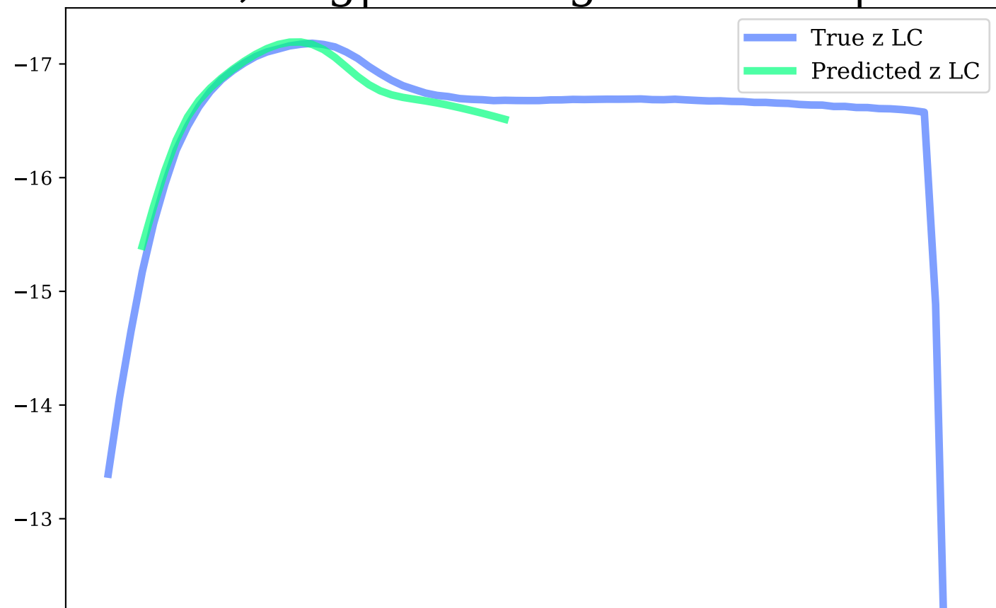
z-band, Avg|Max Mag Diff: 0.09 | 0.23
