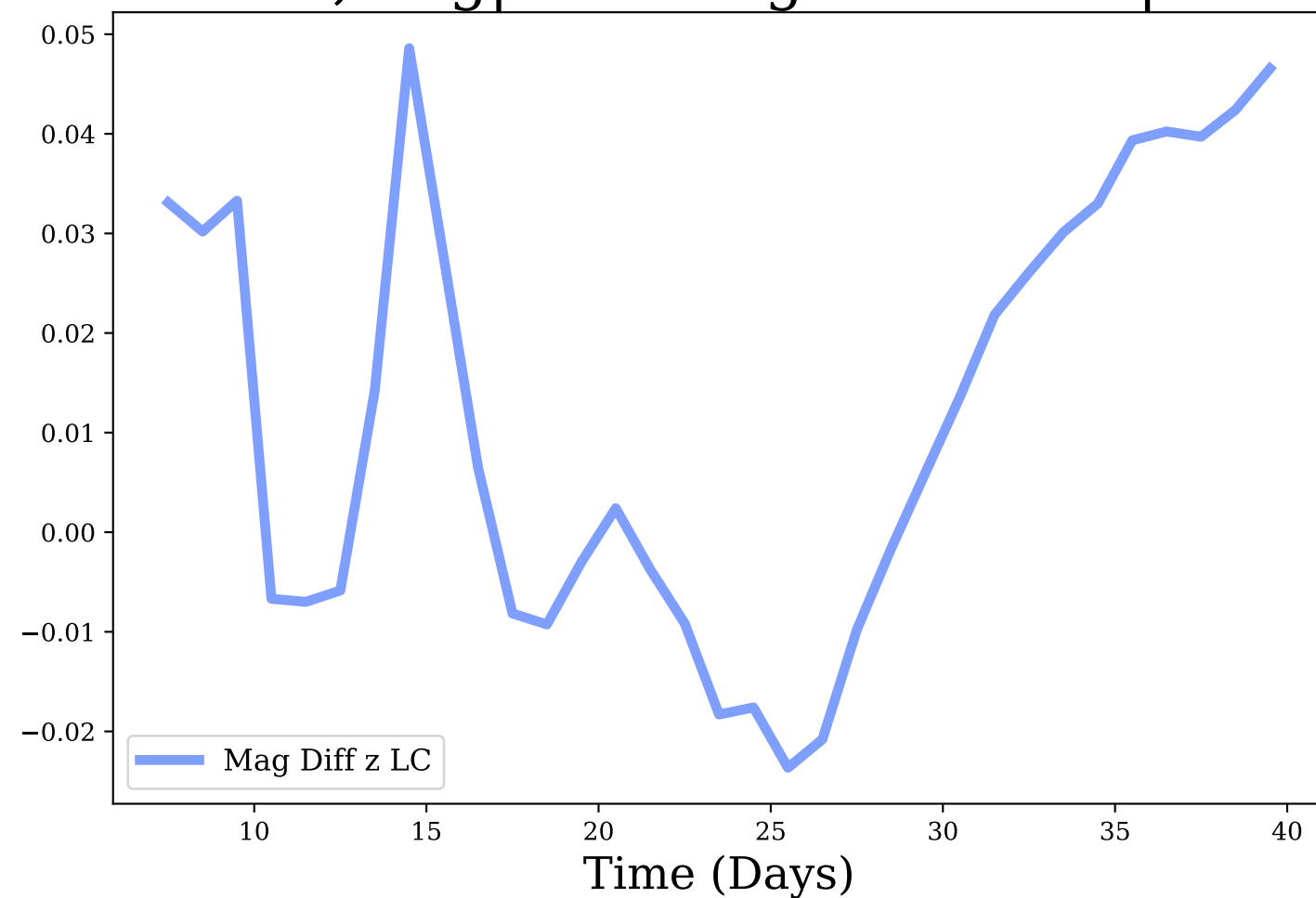
z-band, Avg|Max Mag Diff: 0.01 | 0.05
