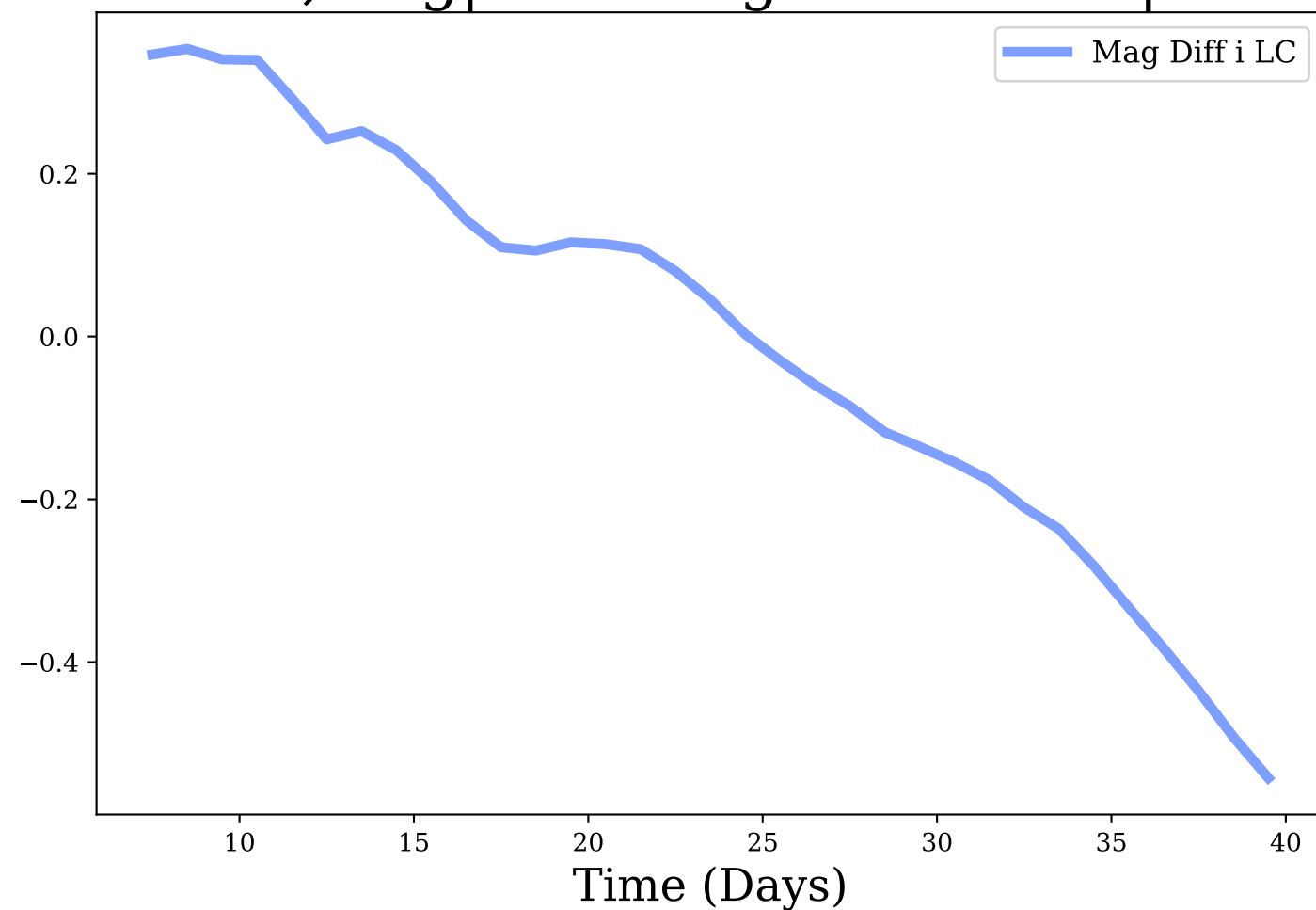
i-band, Avg|Max Mag Diff: -0.01 | 0.54
