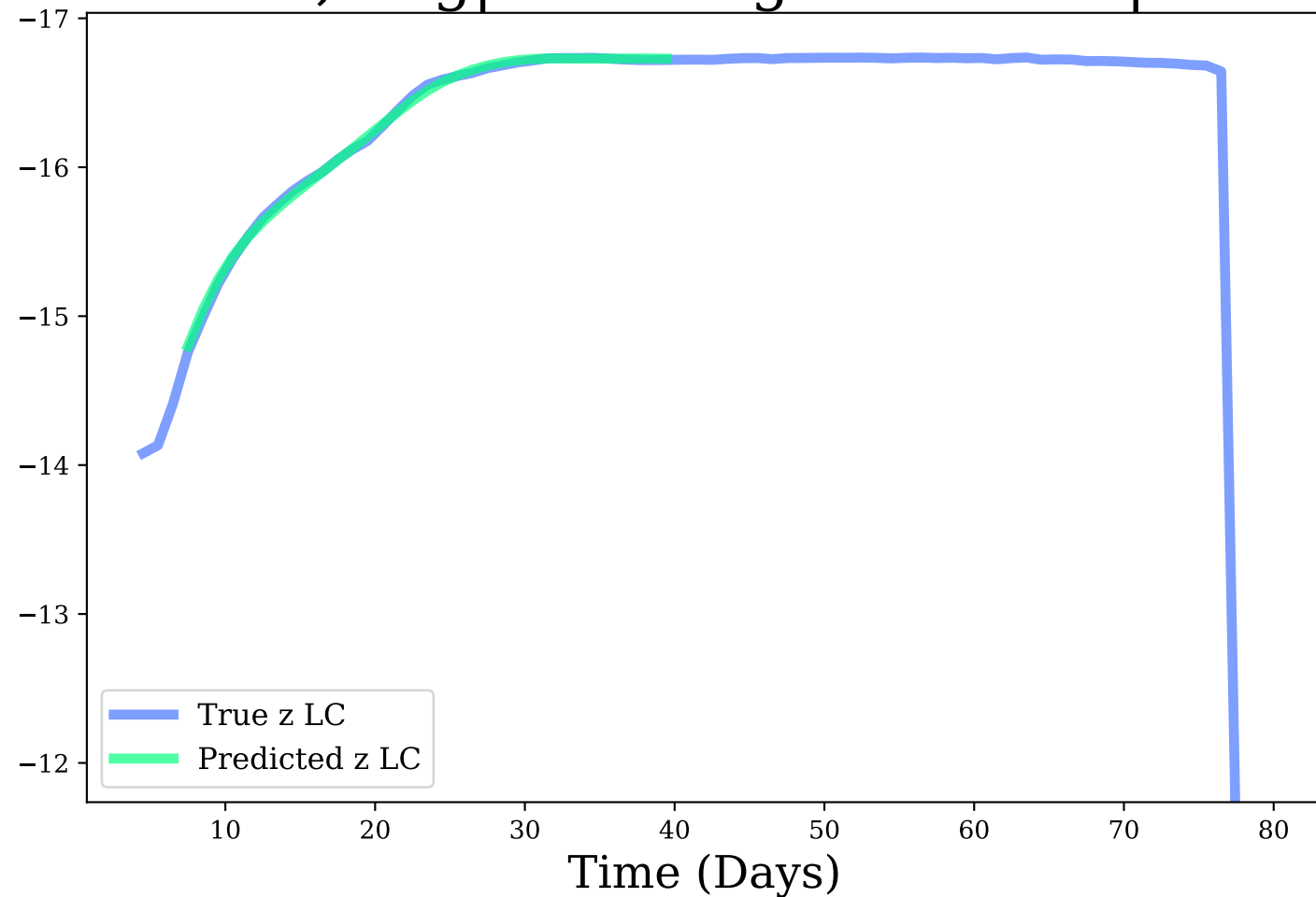
z-band, Avg|Max Mag Diff: 0.02 | 0.05
