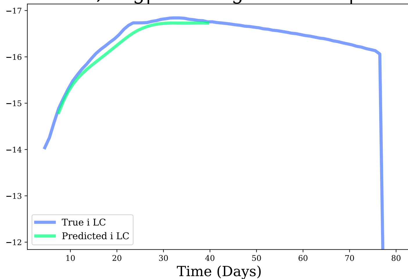
i-band, Avg|Max Mag Diff: 0.12 | 0.23
