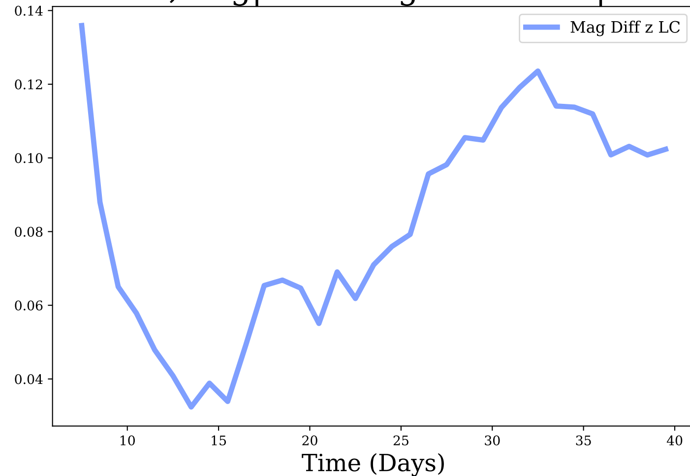
z-band, Avg|Max Mag Diff: 0.08 | 0.14
