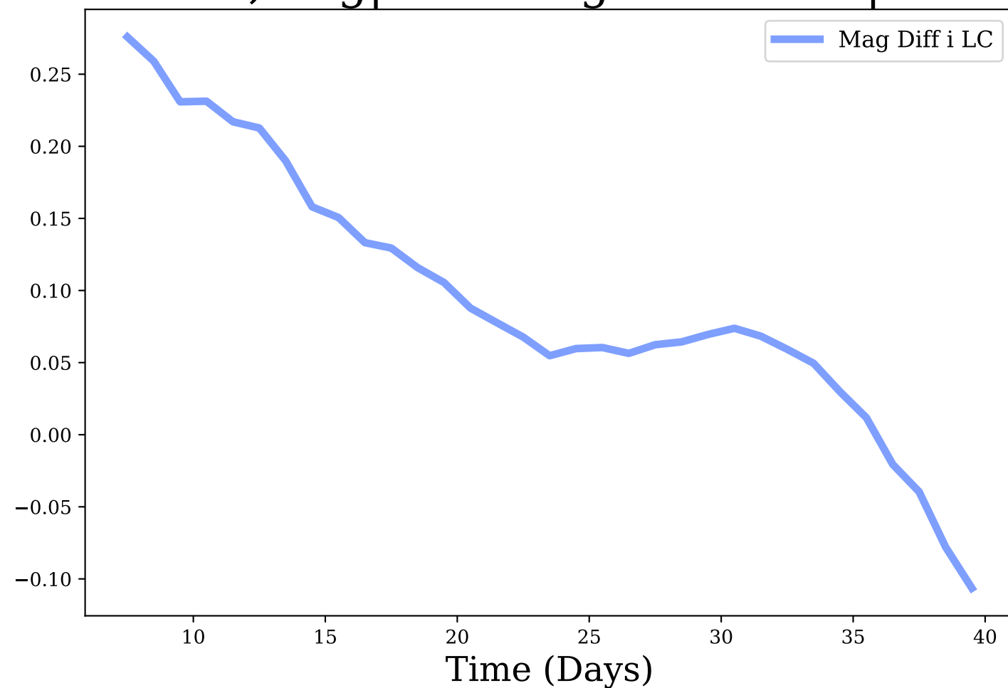
i-band, Avg|Max Mag Diff: 0.09 | 0.28
