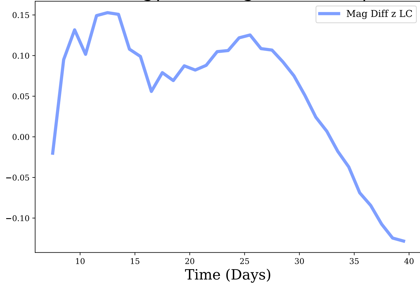
z-band, Avg|Max Mag Diff: 0.05 | 0.15
