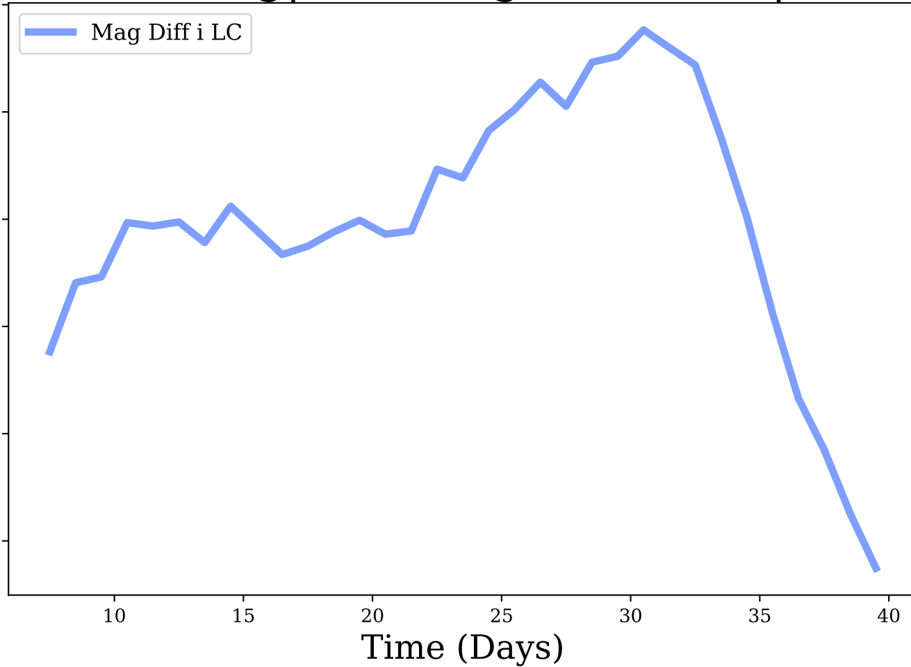
i-band, Avg|Max Mag Diff: 0.25 | 0.34
