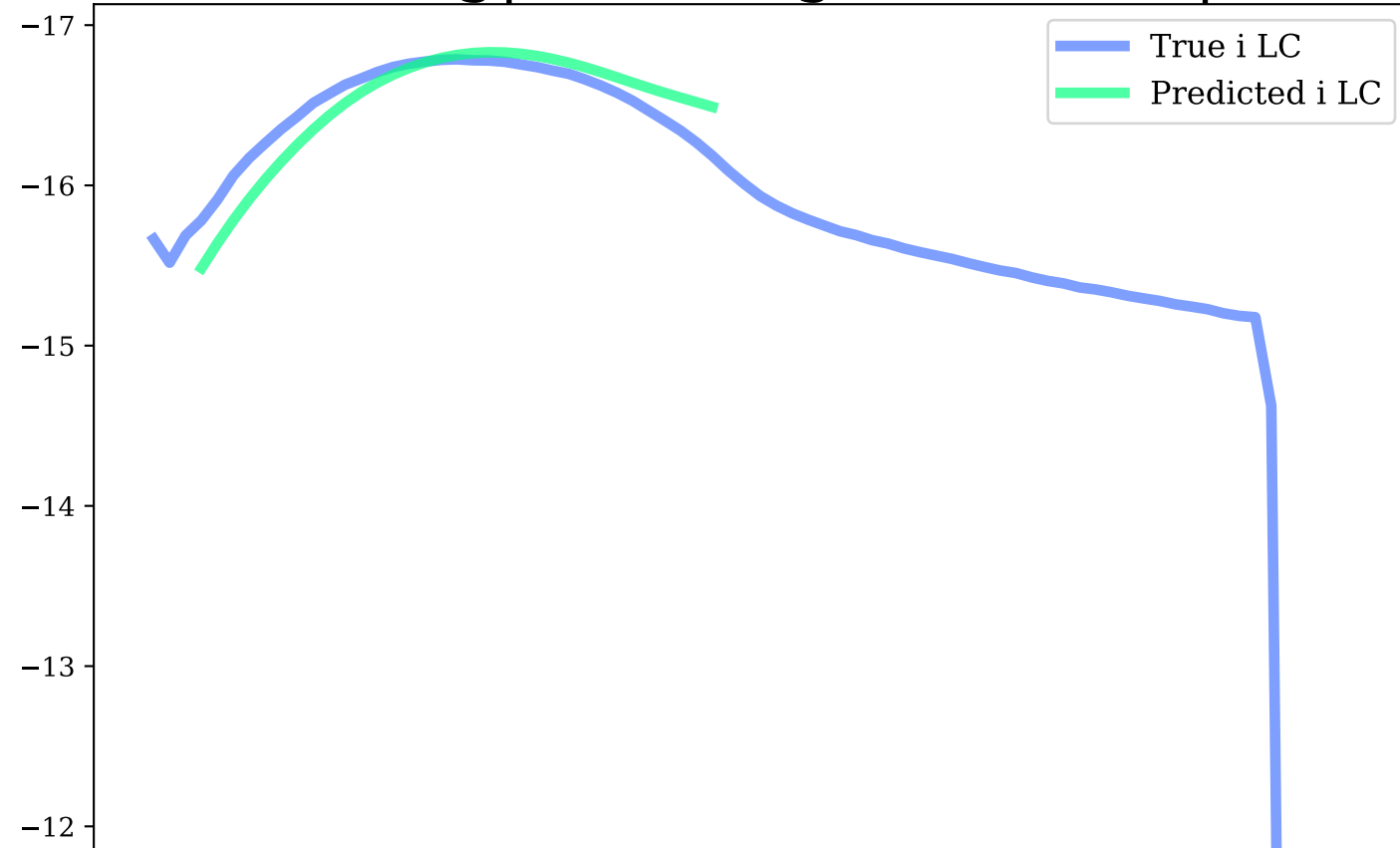
i-band, Avg|Max Mag Diff: 0.13 | 0.31
