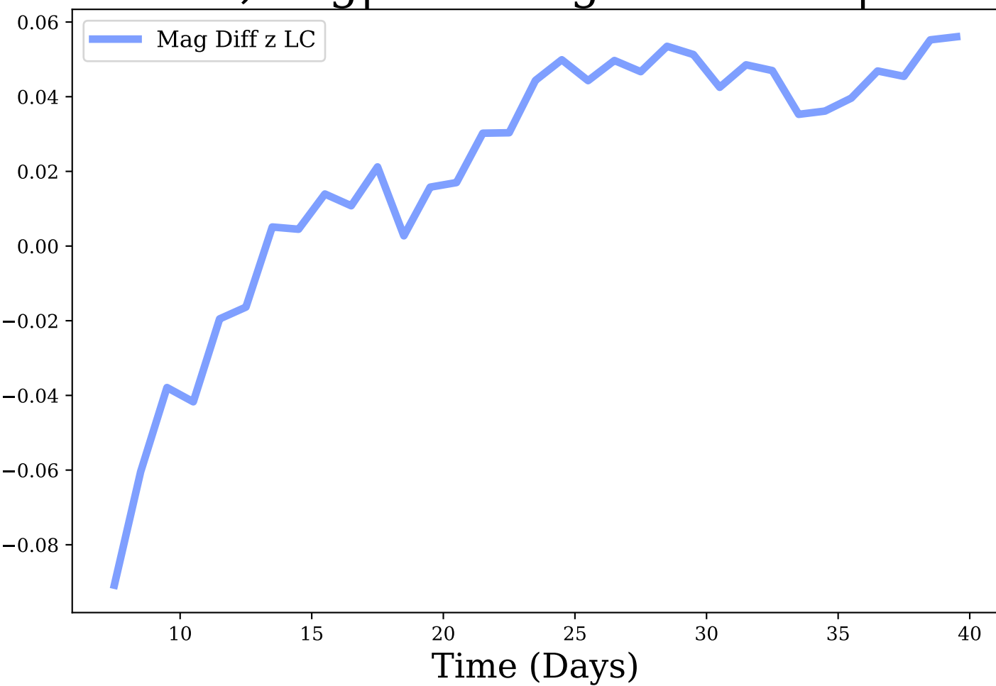
z-band, Avg|Max Mag Diff: 0.02 | 0.09
