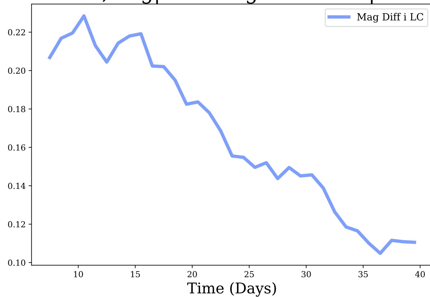
i-band, Avg|Max Mag Diff: 0.17 | 0.23
