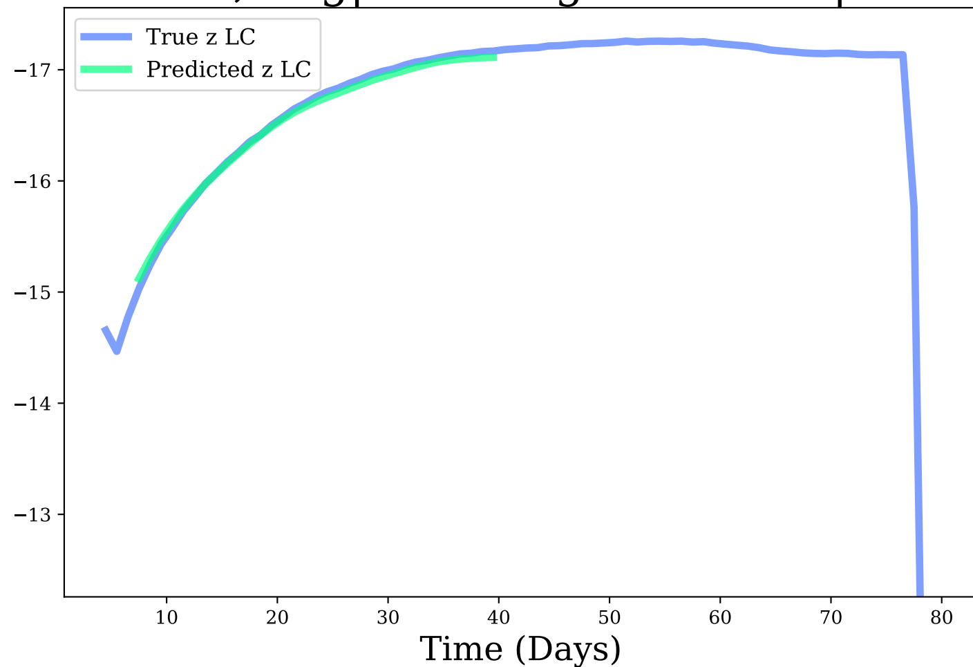
z-band, Avg|Max Mag Diff: 0.04 | 0.09
