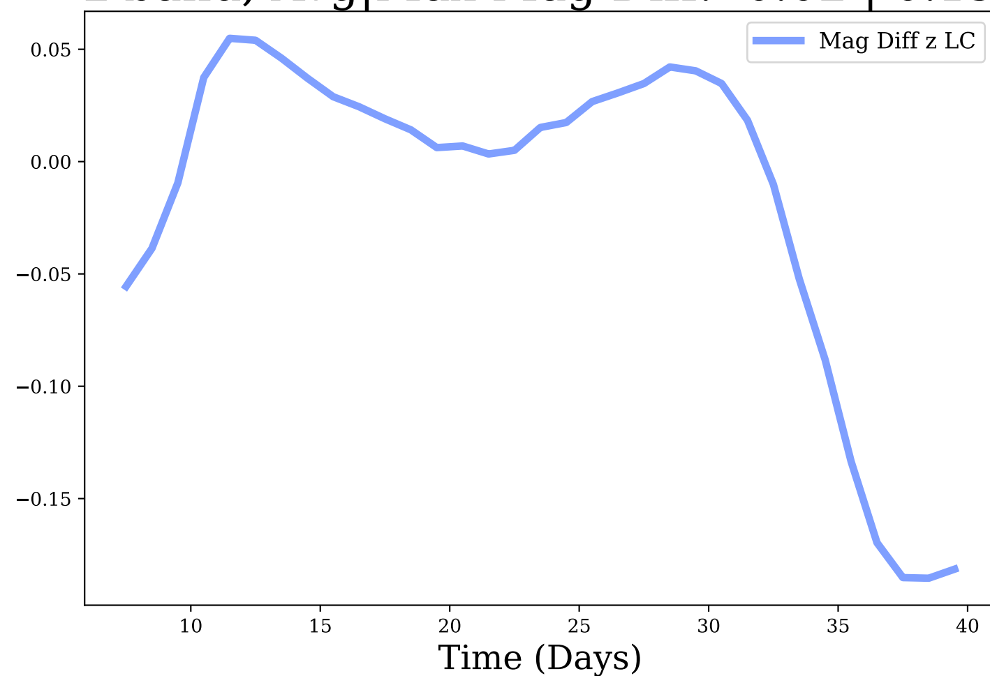
z-band, Avg|Max Mag Diff: -0.02 | 0.19
