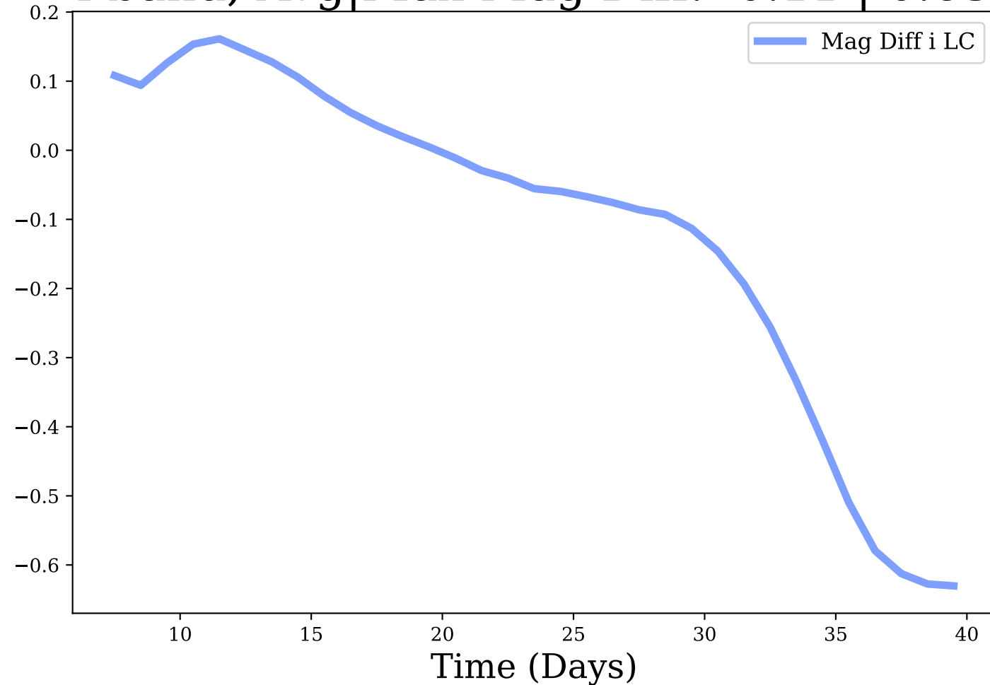
i-band, Avg|Max Mag Diff: -0.11 | 0.63
