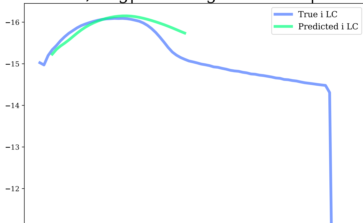
i-band, Avg|Max Mag Diff: 0.19 | 0.63
