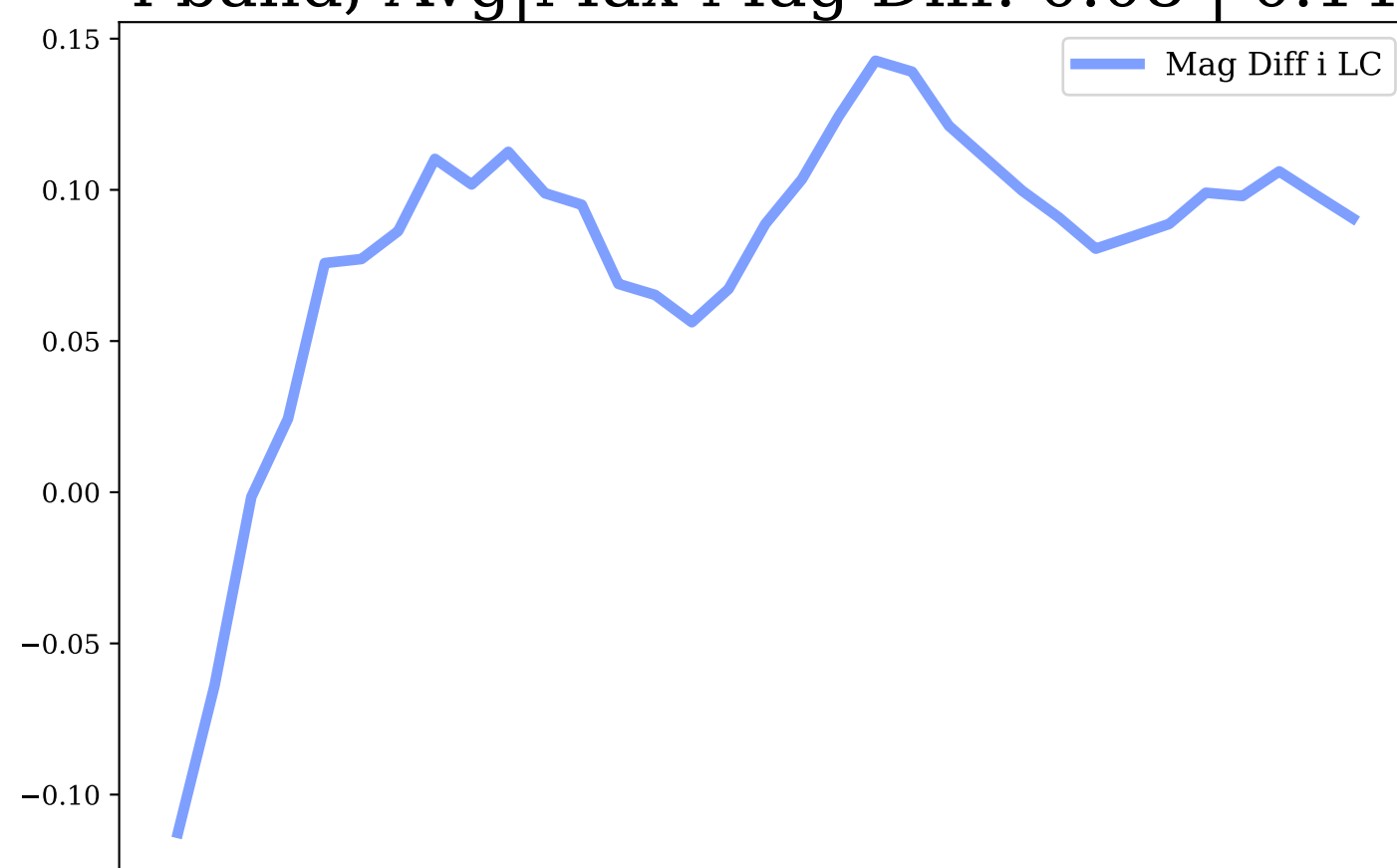
i-band, Avg|Max Mag Diff: 0.08 | 0.14
