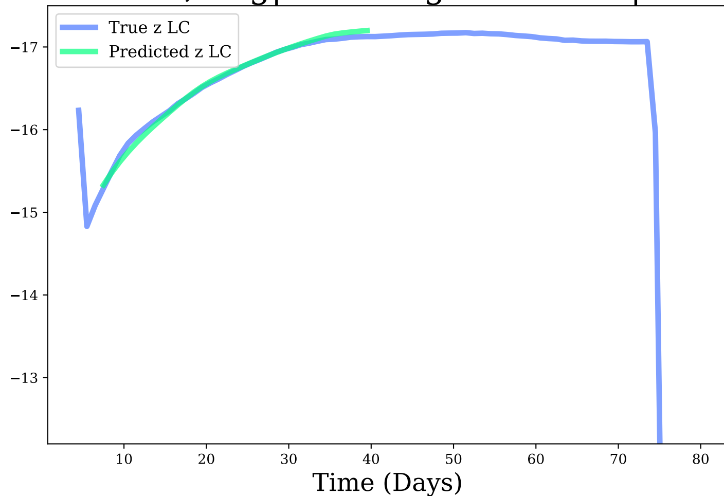
z-band, Avg|Max Mag Diff: 0.03 | 0.1
