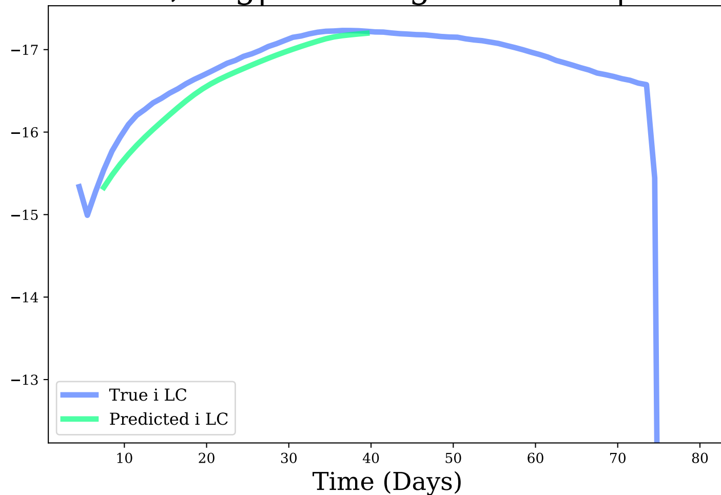
i-band, Avg|Max Mag Diff: 0.18 | 0.36
