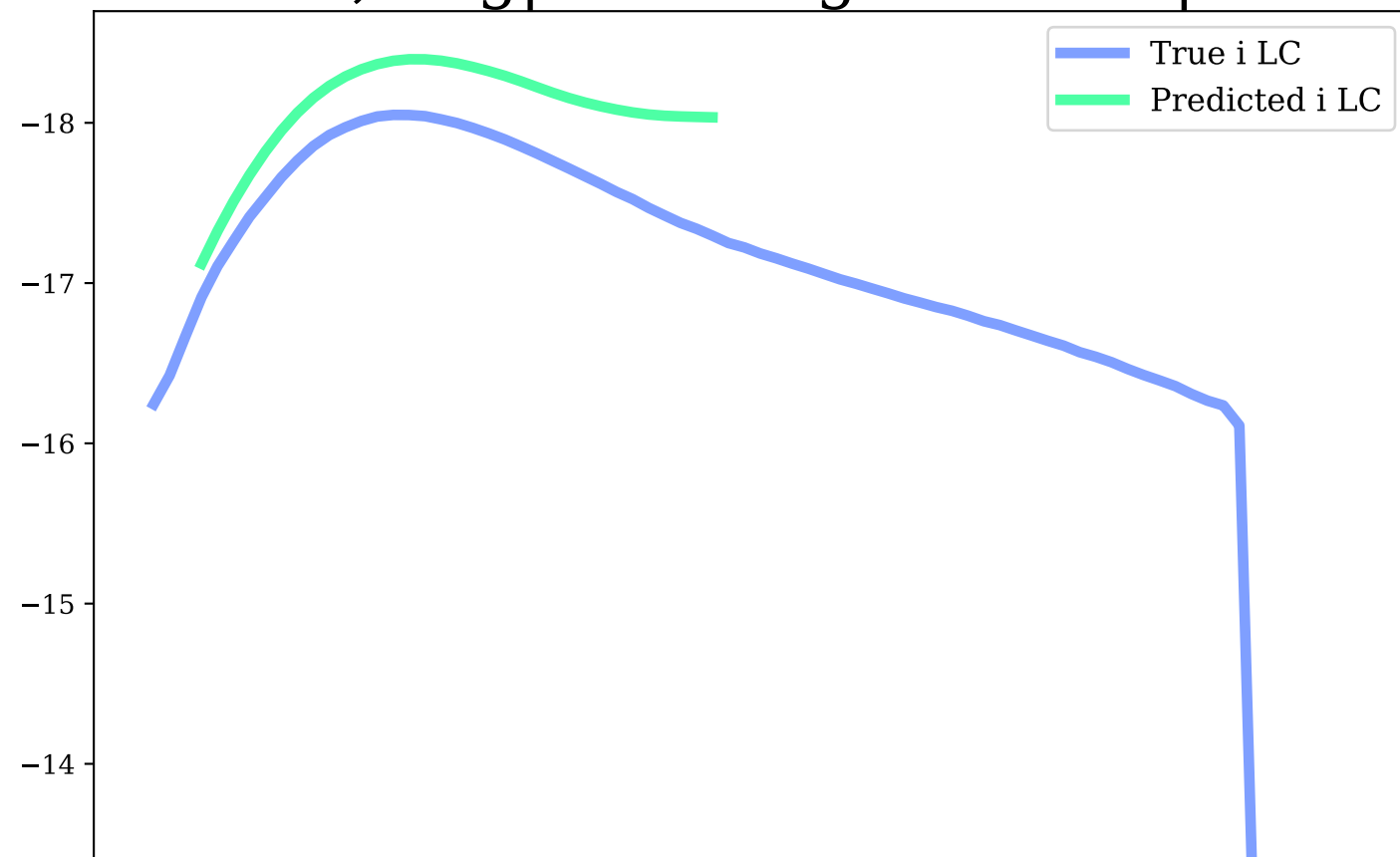
i-band, Avg|Max Mag Diff: 0.4 | 0.74
