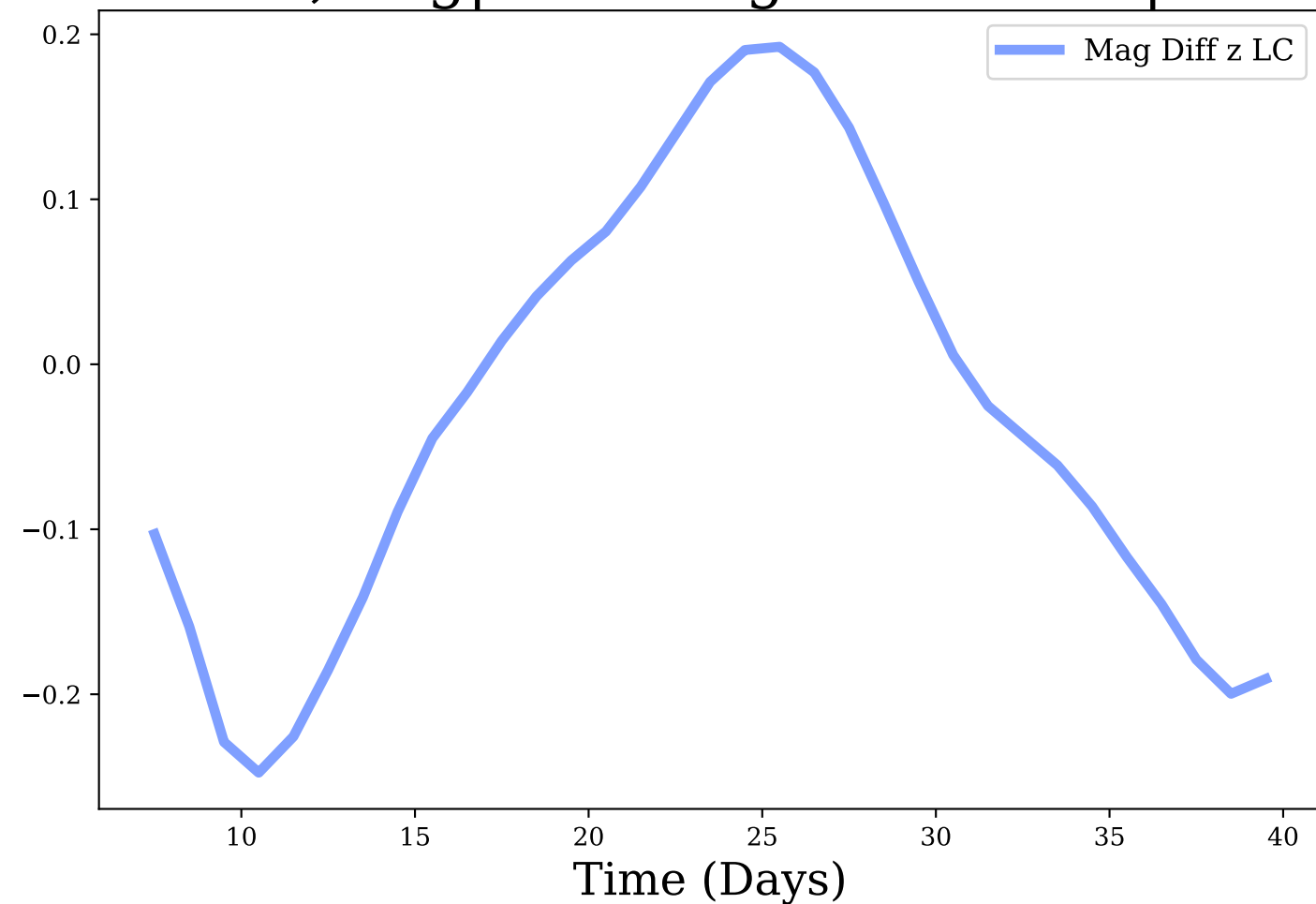
z-band, Avg|Max Mag Diff: -0.03 | 0.25
