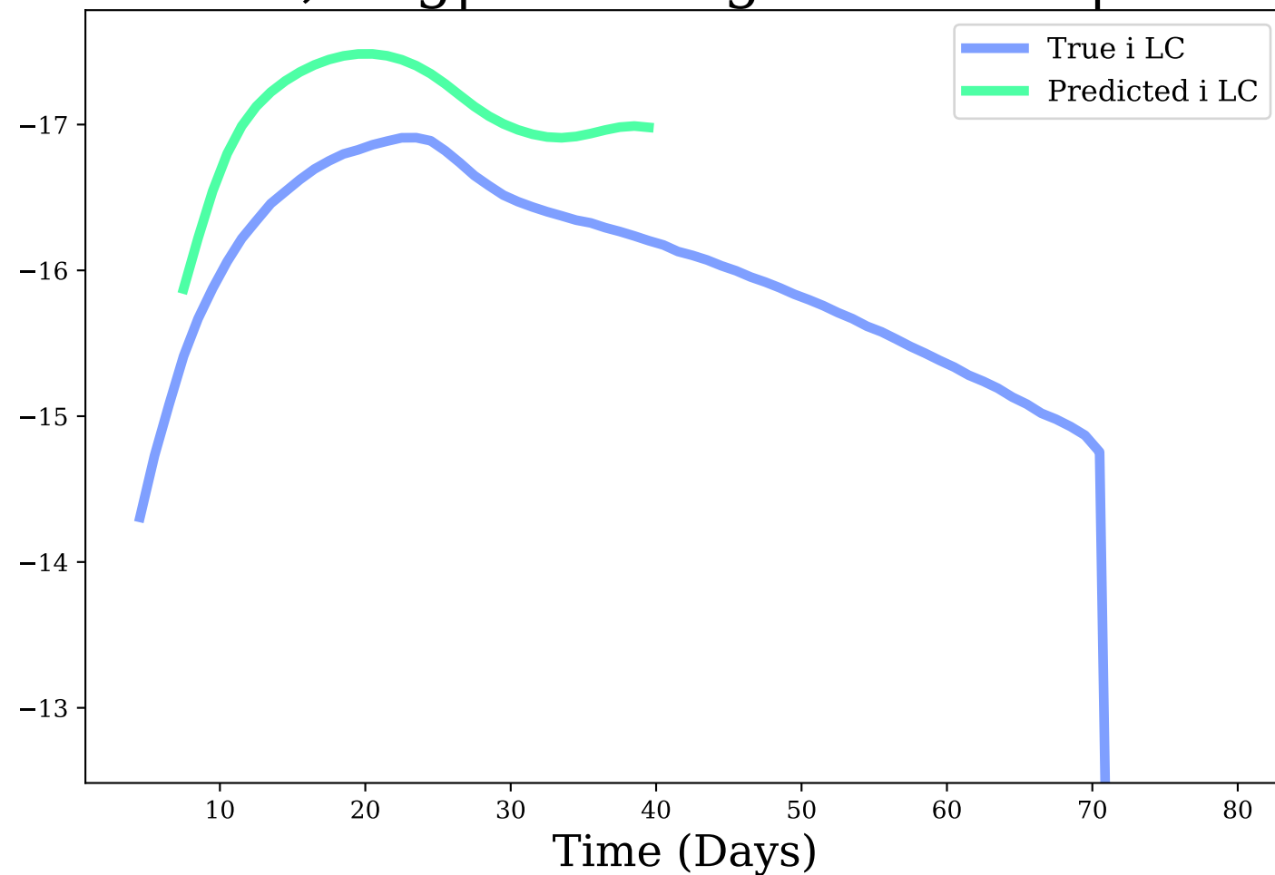
i-band, Avg|Max Mag Diff: 0.61 | 0.78
