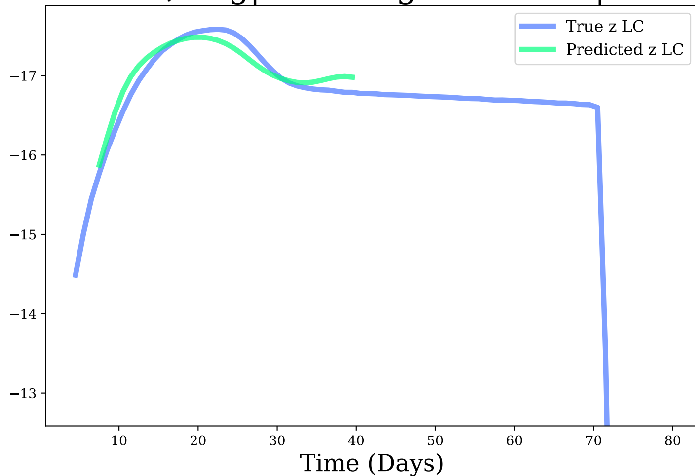
z-band, Avg|Max Mag Diff: 0.12 | 0.25
