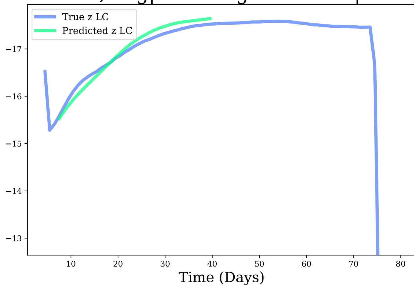
z-band, Avg|Max Mag Diff: 0.12 | 0.19
