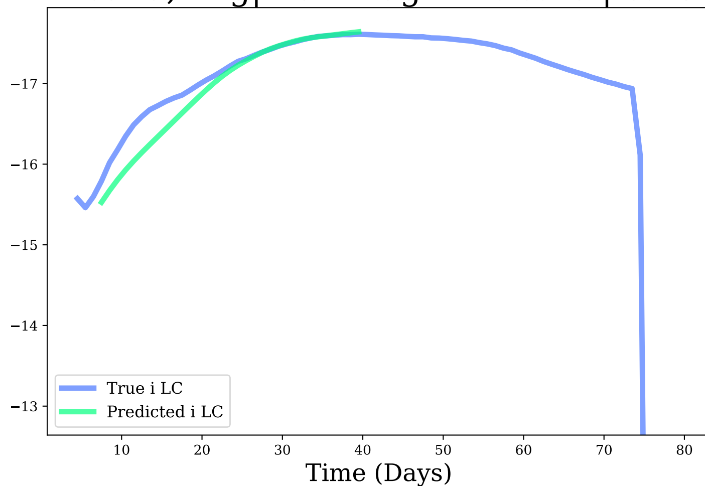
i-band, Avg|Max Mag Diff: 0.15 | 0.45
