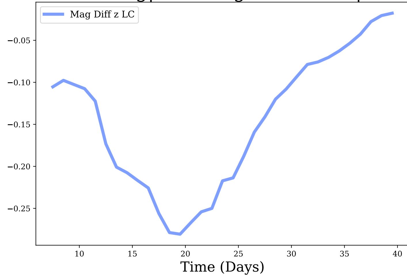
z-band, Avg|Max Mag Diff: -0.15 | 0.28
