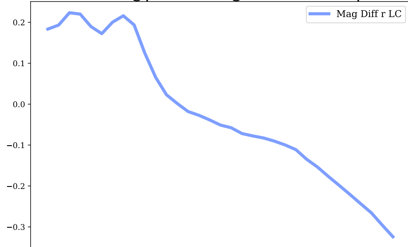
r-band, Avg|Max Mag Diff: -0.02 | 0.32
