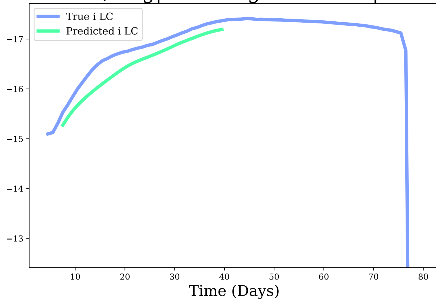
i-band, Avg|Max Mag Diff: 0.27 | 0.46
