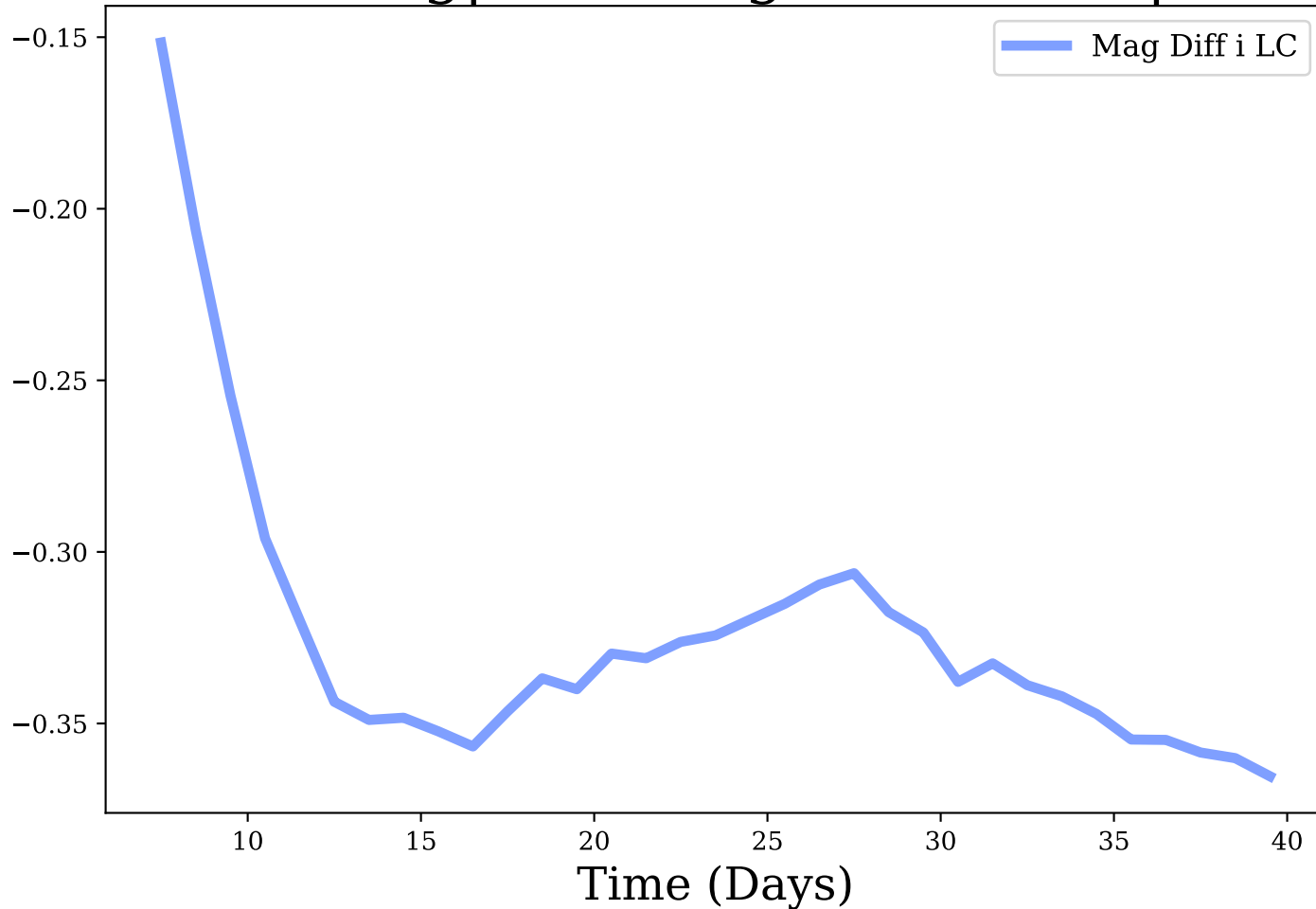
i-band, Avg|Max Mag Diff: -0.32 | 0.37
