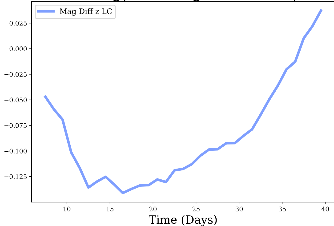
z-band, Avg|Max Mag Diff: -0.09 | 0.14
