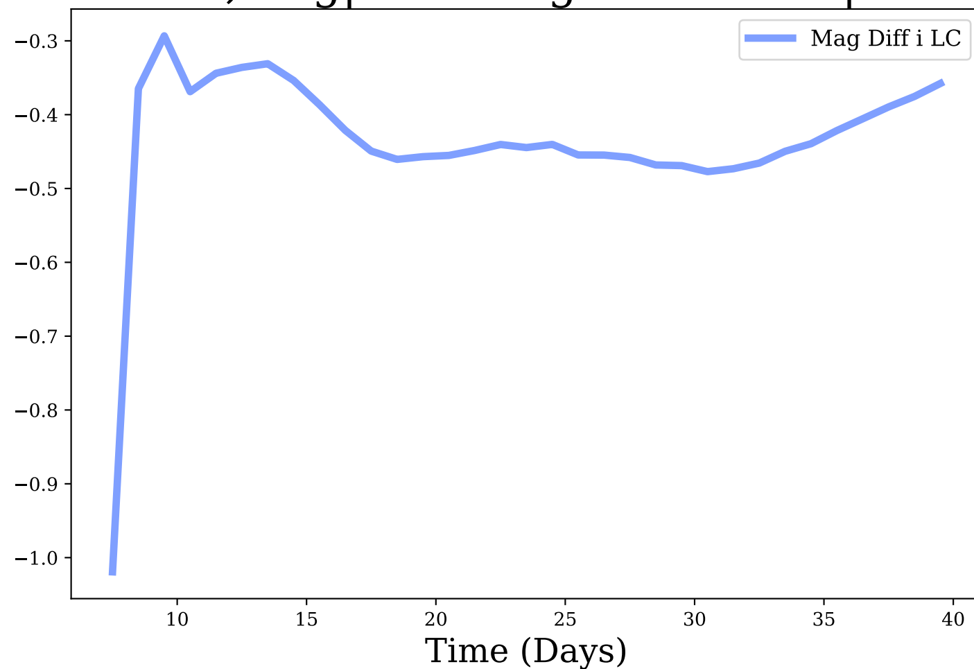
i-band, Avg|Max Mag Diff: -0.44 | 1.02
