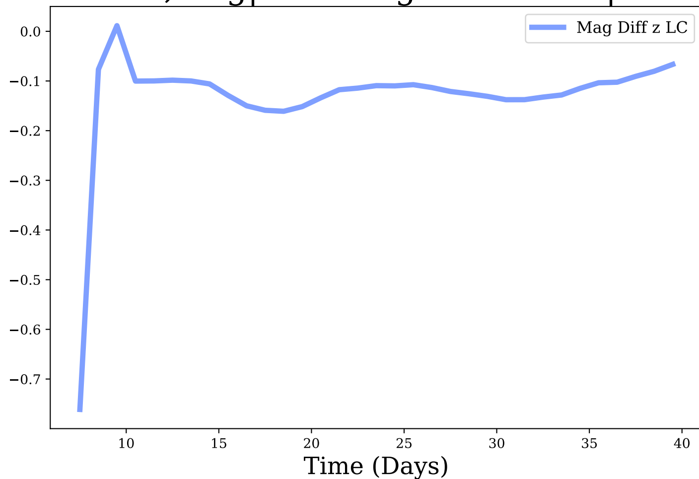
z-band, Avg|Max Mag Diff: -0.13 | 0.76
