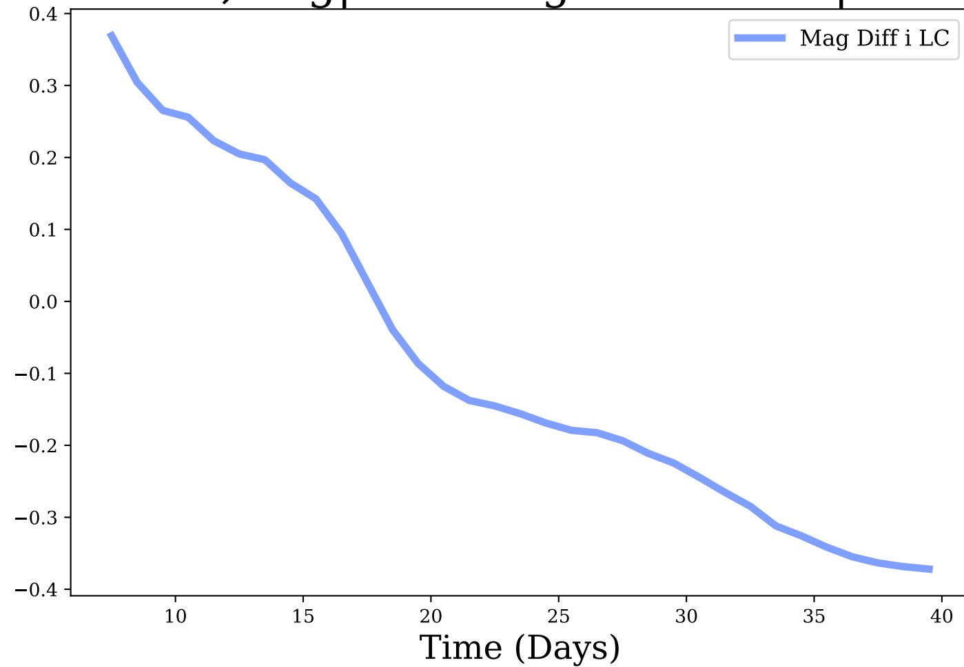
i-band, Avg|Max Mag Diff: -0.09 | 0.37
