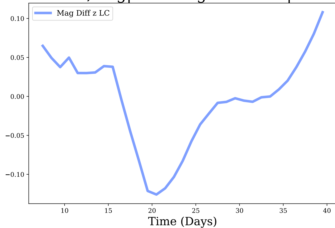
z-band, Avg|Max Mag Diff: -0.0 | 0.13
