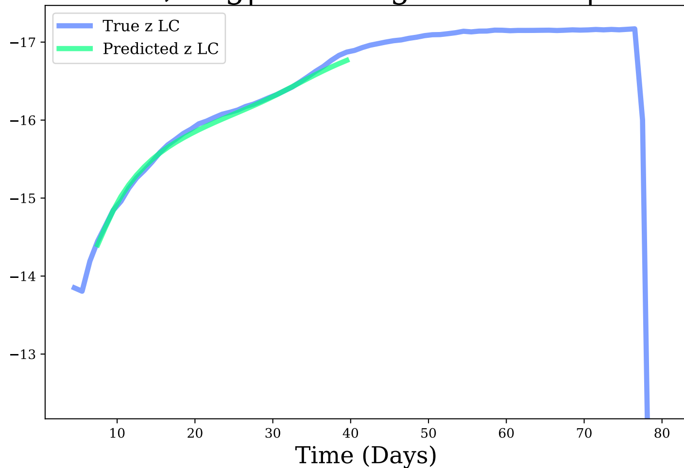
z-band, Avg|Max Mag Diff: 0.04 | 0.11
