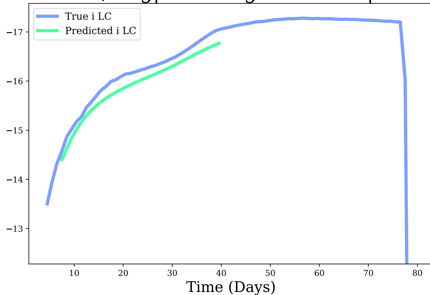
i-band, Avg|Max Mag Diff: 0.21 | 0.28
