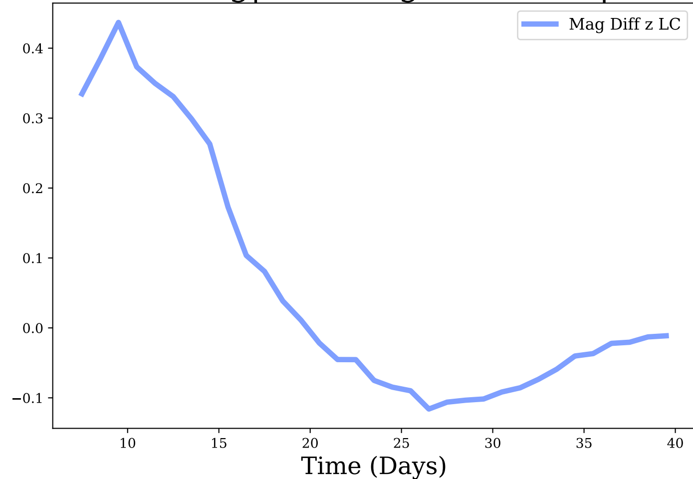
z-band, Avg|Max Mag Diff: 0.06 | 0.44
