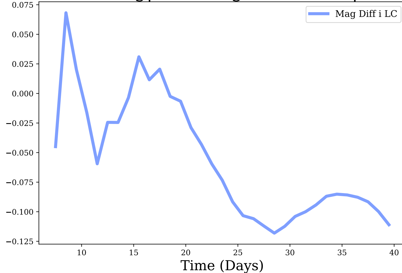
i-band, Avg|Max Mag Diff: -0.06 | 0.12
