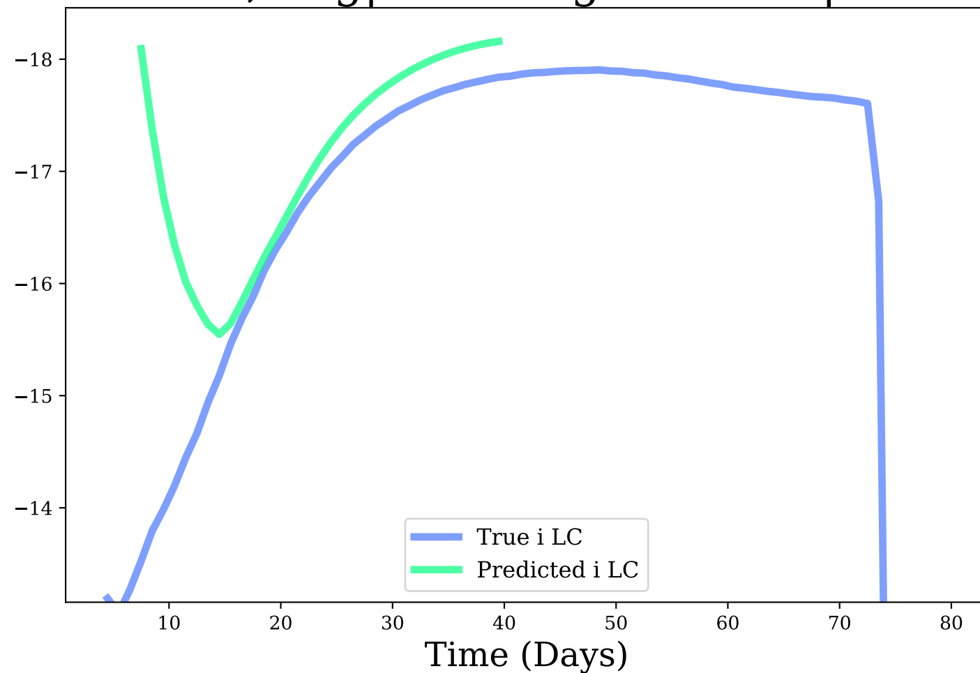
i-band, Avg|Max Mag Diff: 0.7 | 4.57
