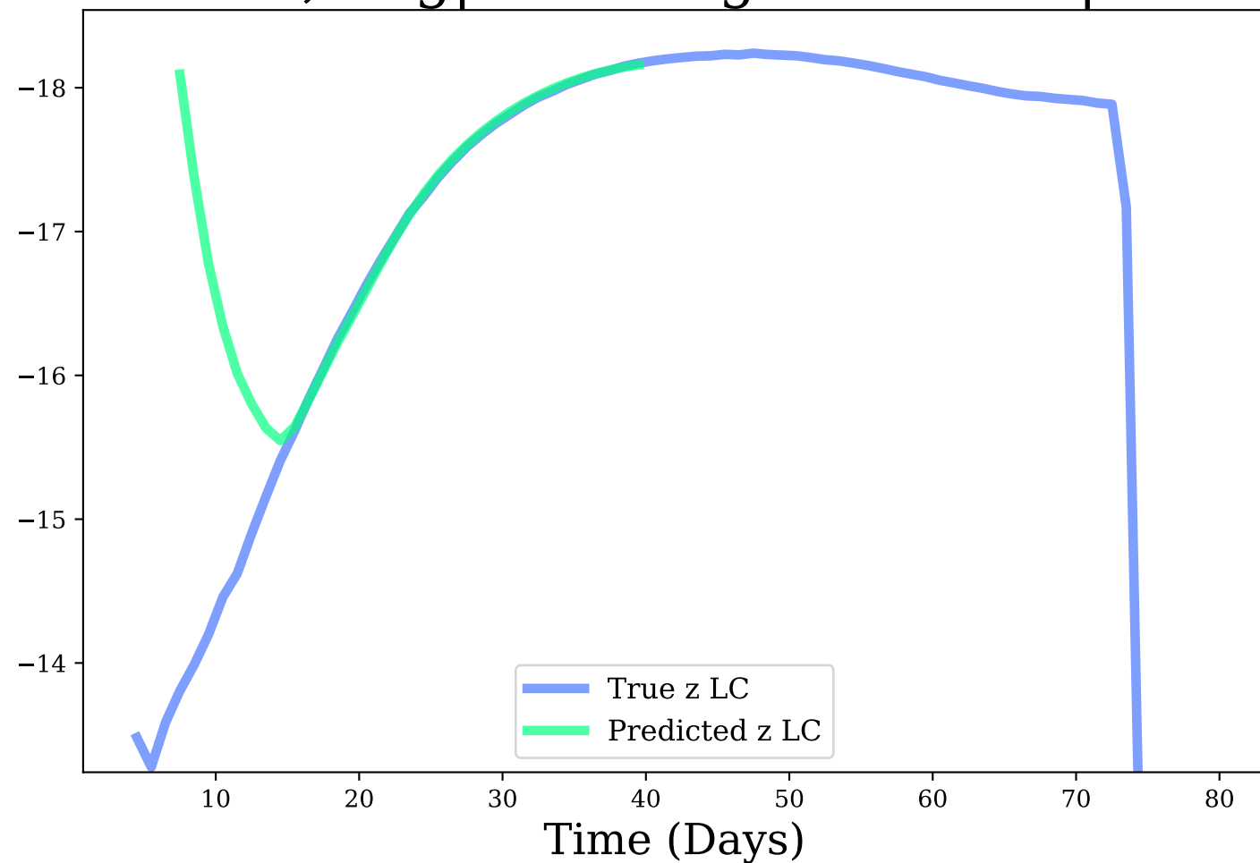
z-band, Avg|Max Mag Diff: 0.47 | 4.29
