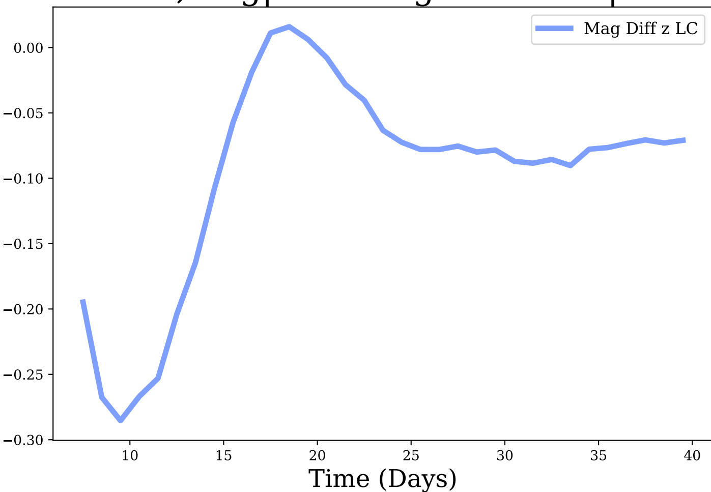
z-band, Avg|Max Mag Diff: -0.1 | 0.29
