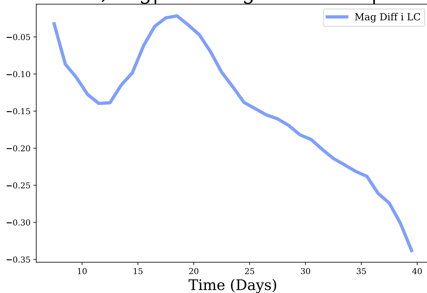
i-band, Avg|Max Mag Diff: -0.14 | 0.34
