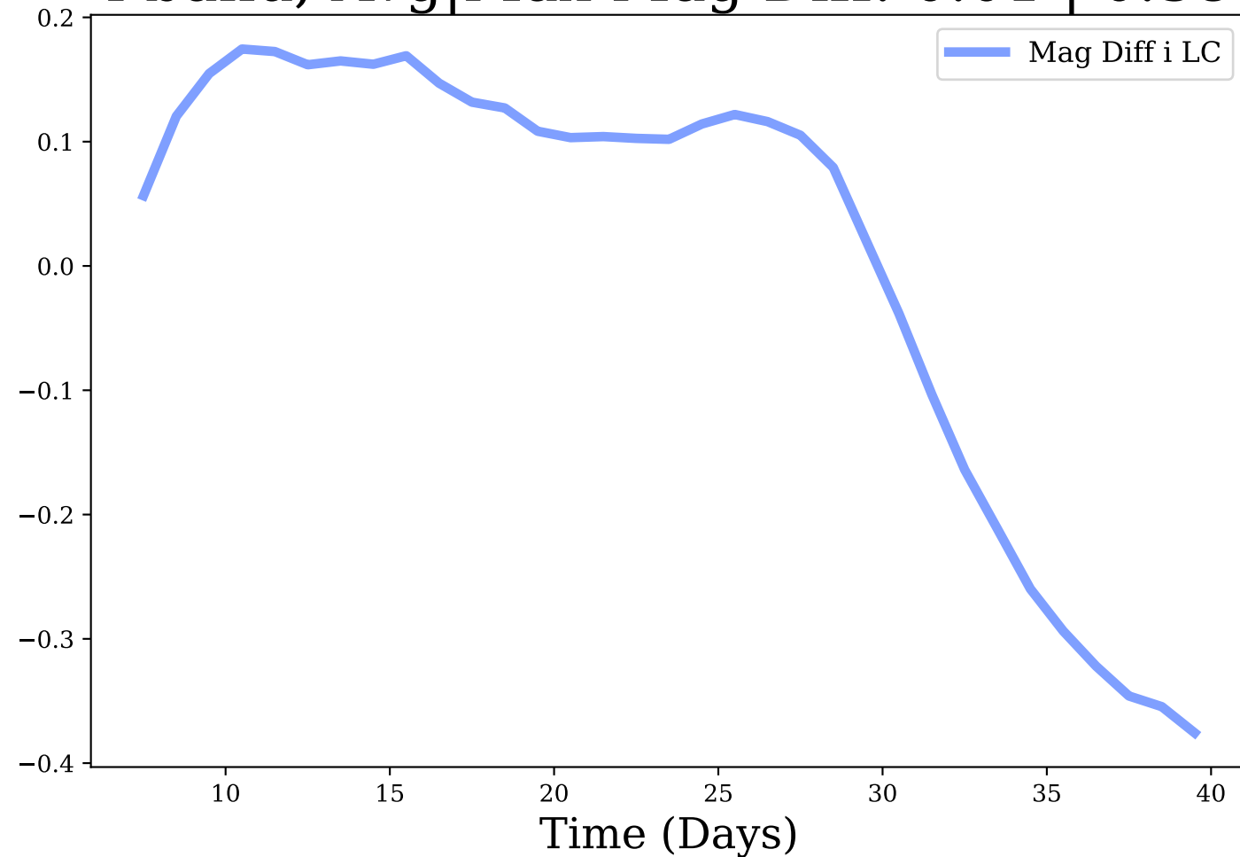
i-band, Avg|Max Mag Diff: 0.01 | 0.38
