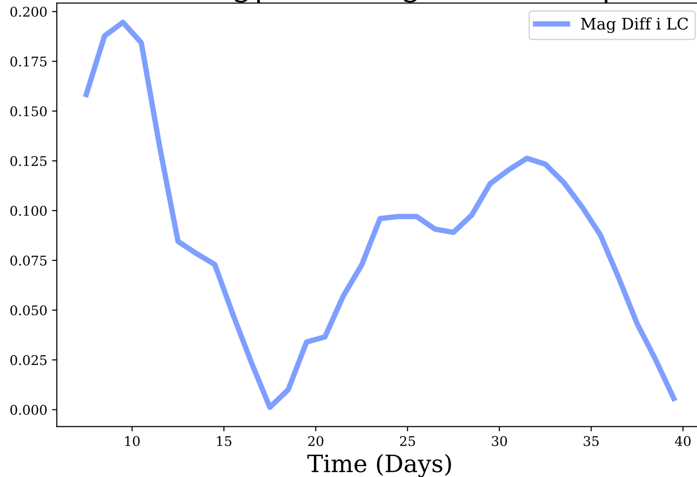
i-band, Avg|Max Mag Diff: 0.09 | 0.19
