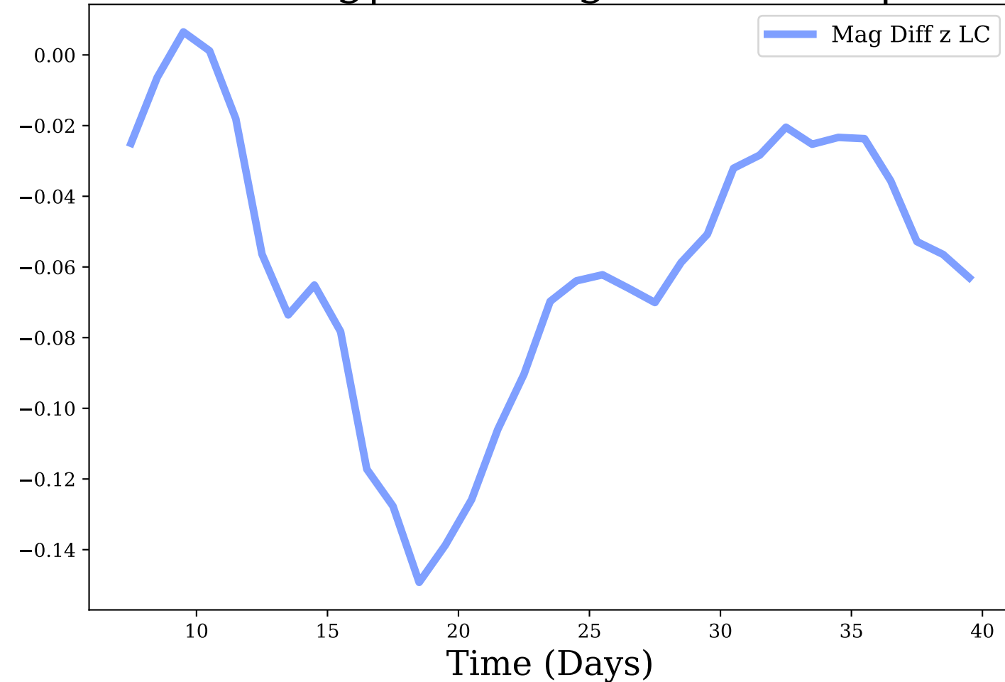
z-band, Avg|Max Mag Diff: -0.06 | 0.15
