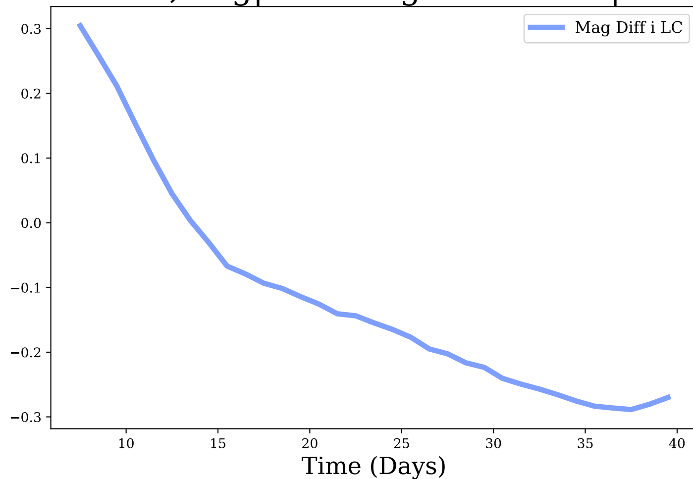
i-band, Avg|Max Mag Diff: -0.12 | 0.3
