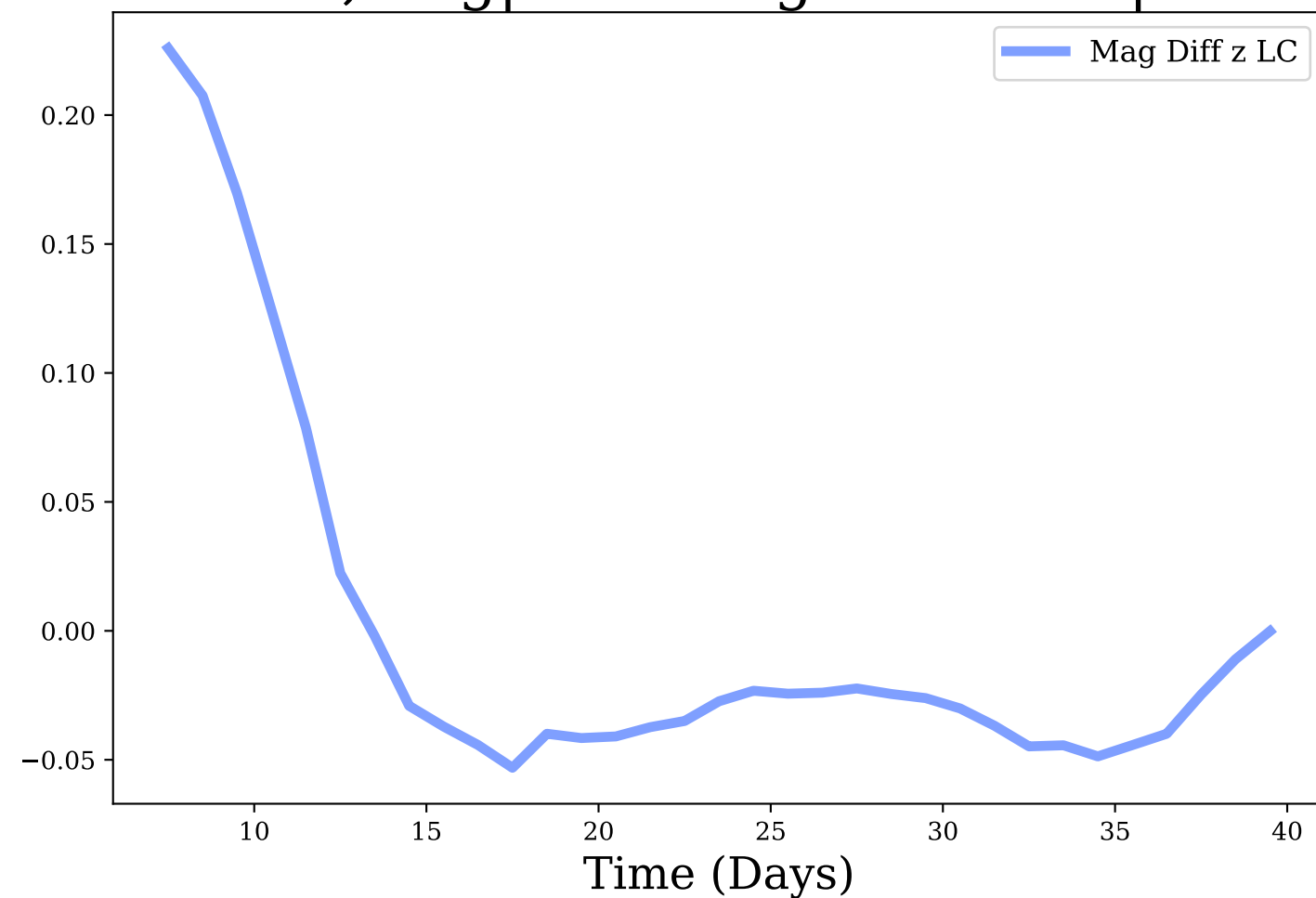
z-band, Avg|Max Mag Diff: -0.0 | 0.23
