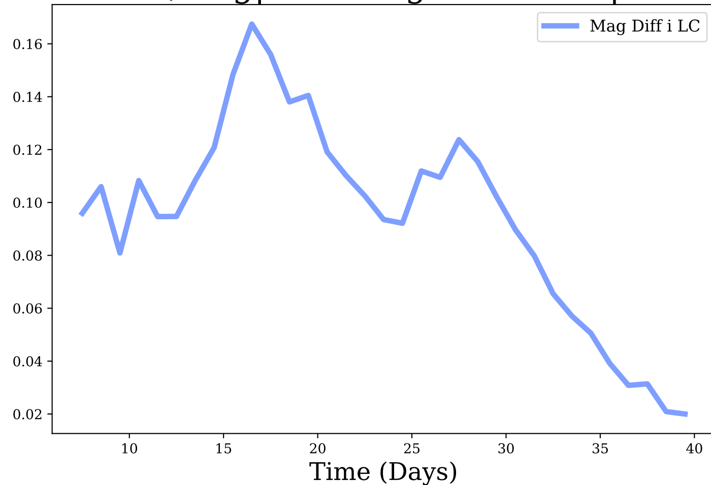
i-band, Avg|Max Mag Diff: 0.09 | 0.17
