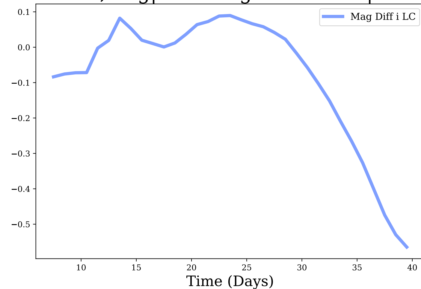
i-band, Avg|Max Mag Diff: -0.08 | 0.56
