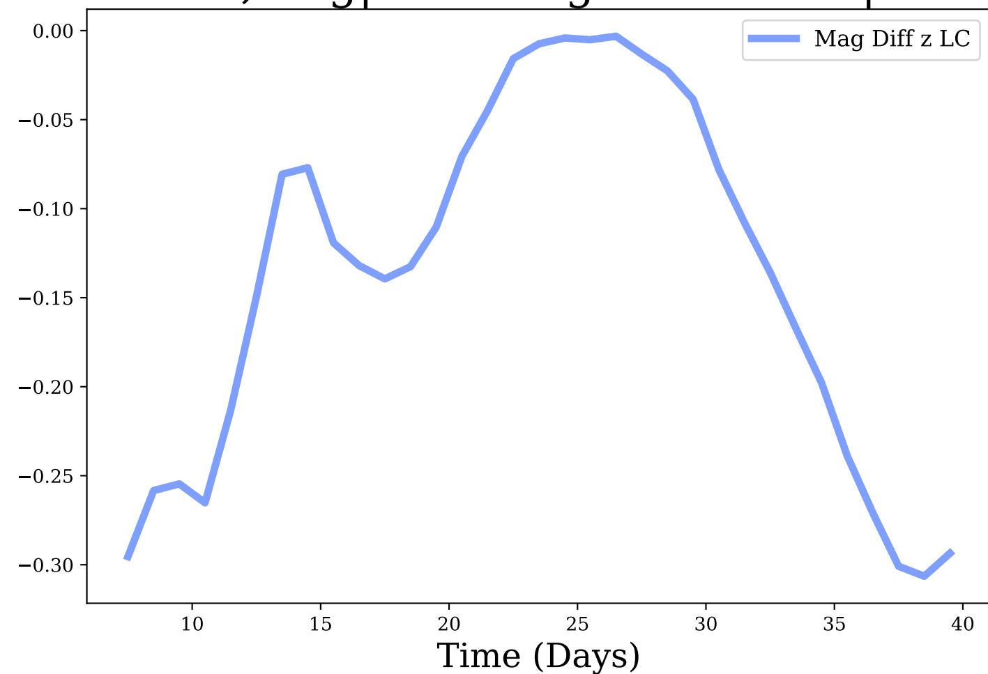
z-band, Avg|Max Mag Diff: -0.14 | 0.31
