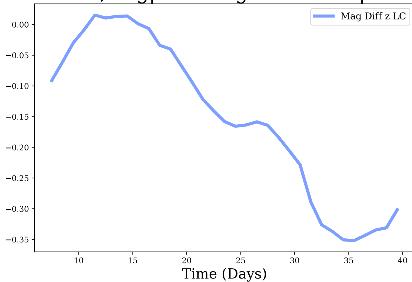
z-band, Avg|Max Mag Diff: -0.15 | 0.35
