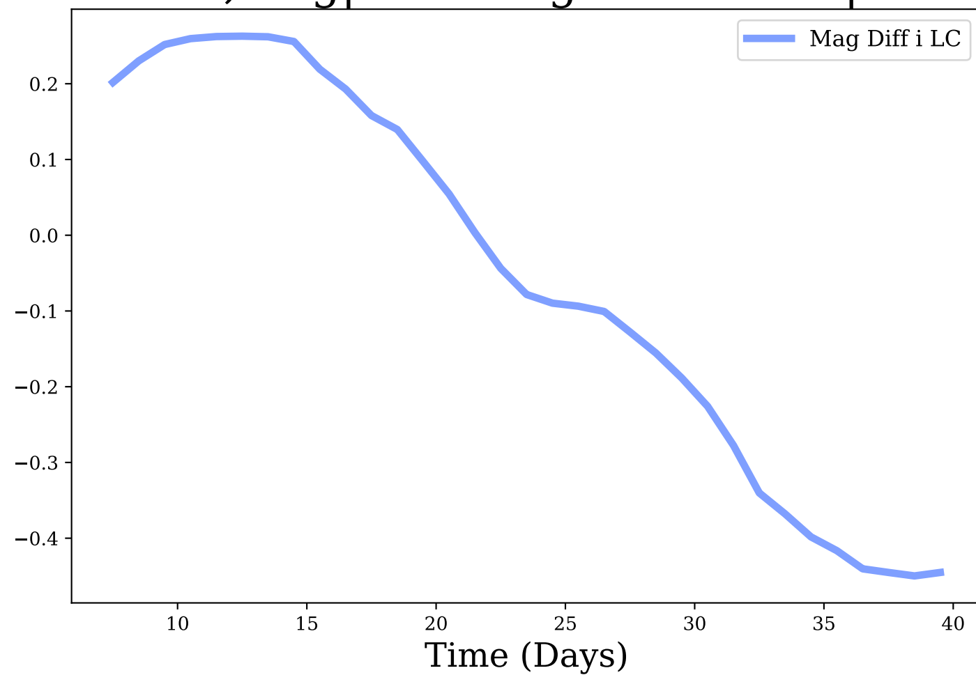
i-band, Avg|Max Mag Diff: -0.06 | 0.45
