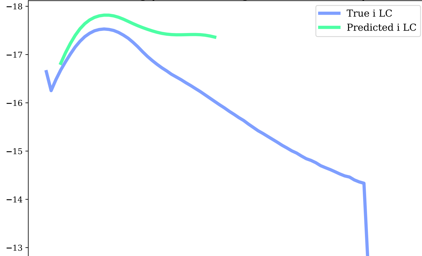
i-band, Avg|Max Mag Diff: 0.59 | 1.33
