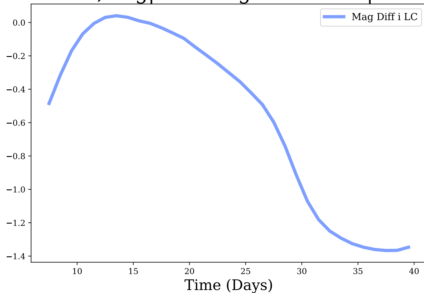
i-band, Avg|Max Mag Diff: -0.56 | 1.37
