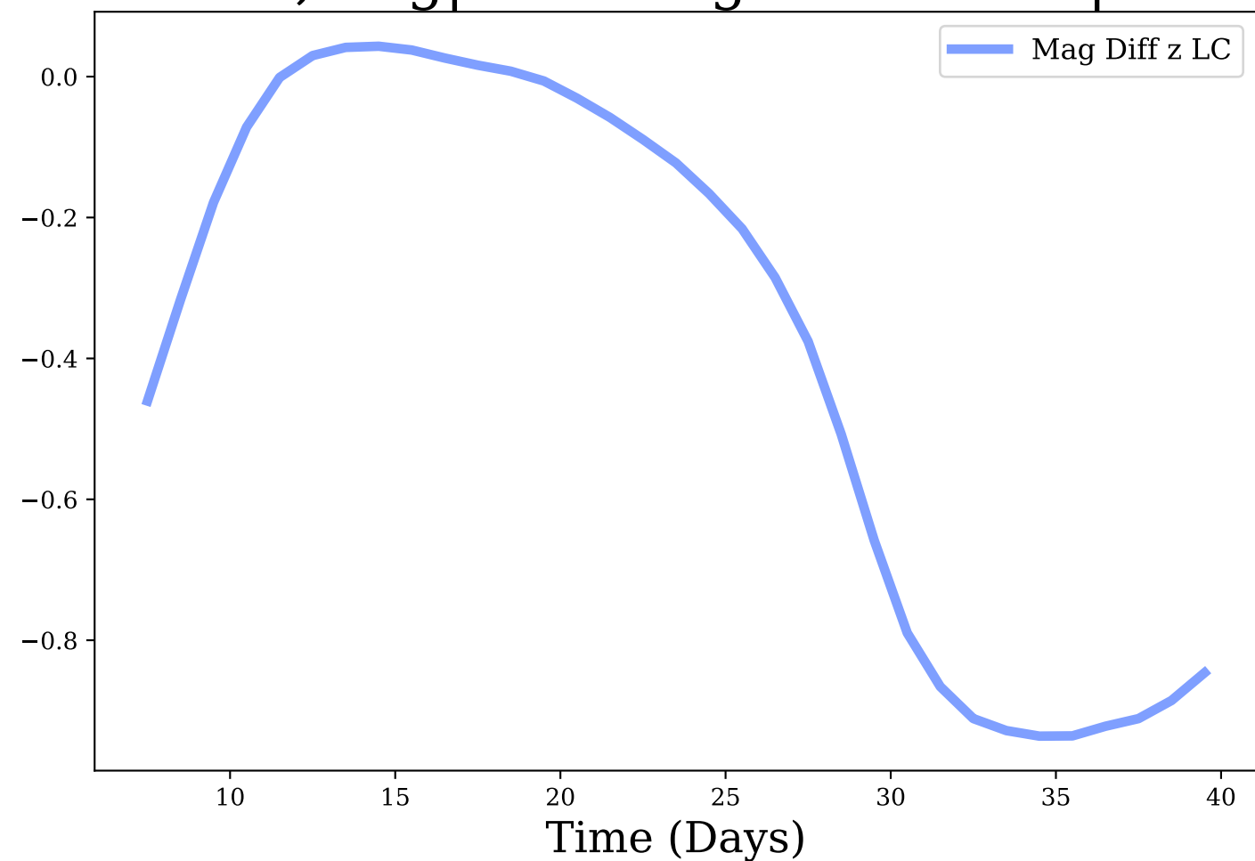
z-band, Avg|Max Mag Diff: -0.37 | 0.94
