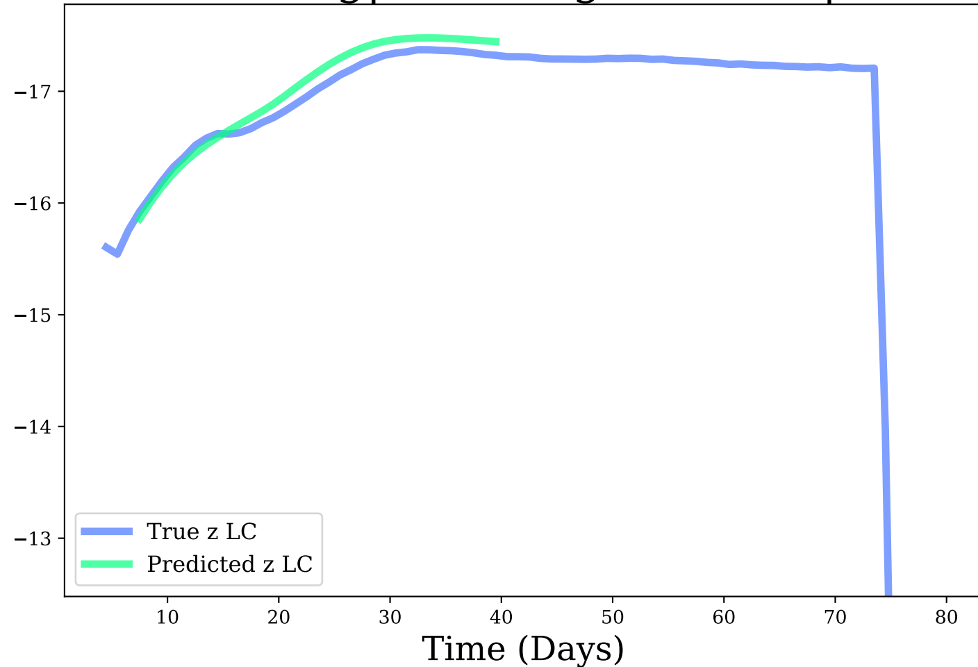
z-band, Avg|Max Mag Diff: 0.1 | 0.16
