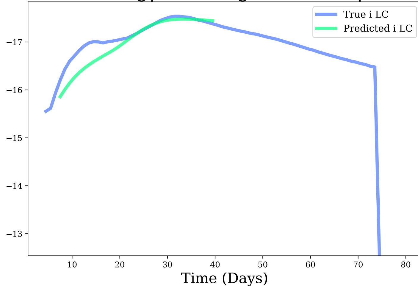
i-band, Avg|Max Mag Diff: 0.16 | 0.47
