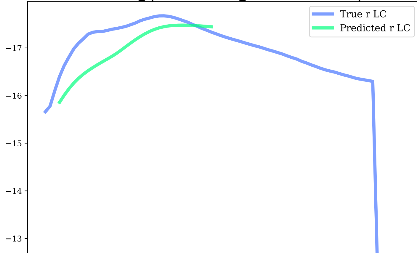
z-band, Avg|Max Mag Diff: 0.1 | 0.16
