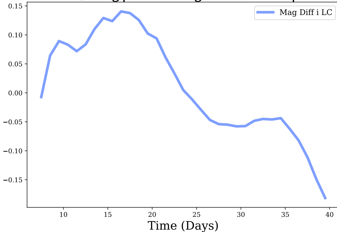
i-band, Avg|Max Mag Diff: 0.01 | 0.18
