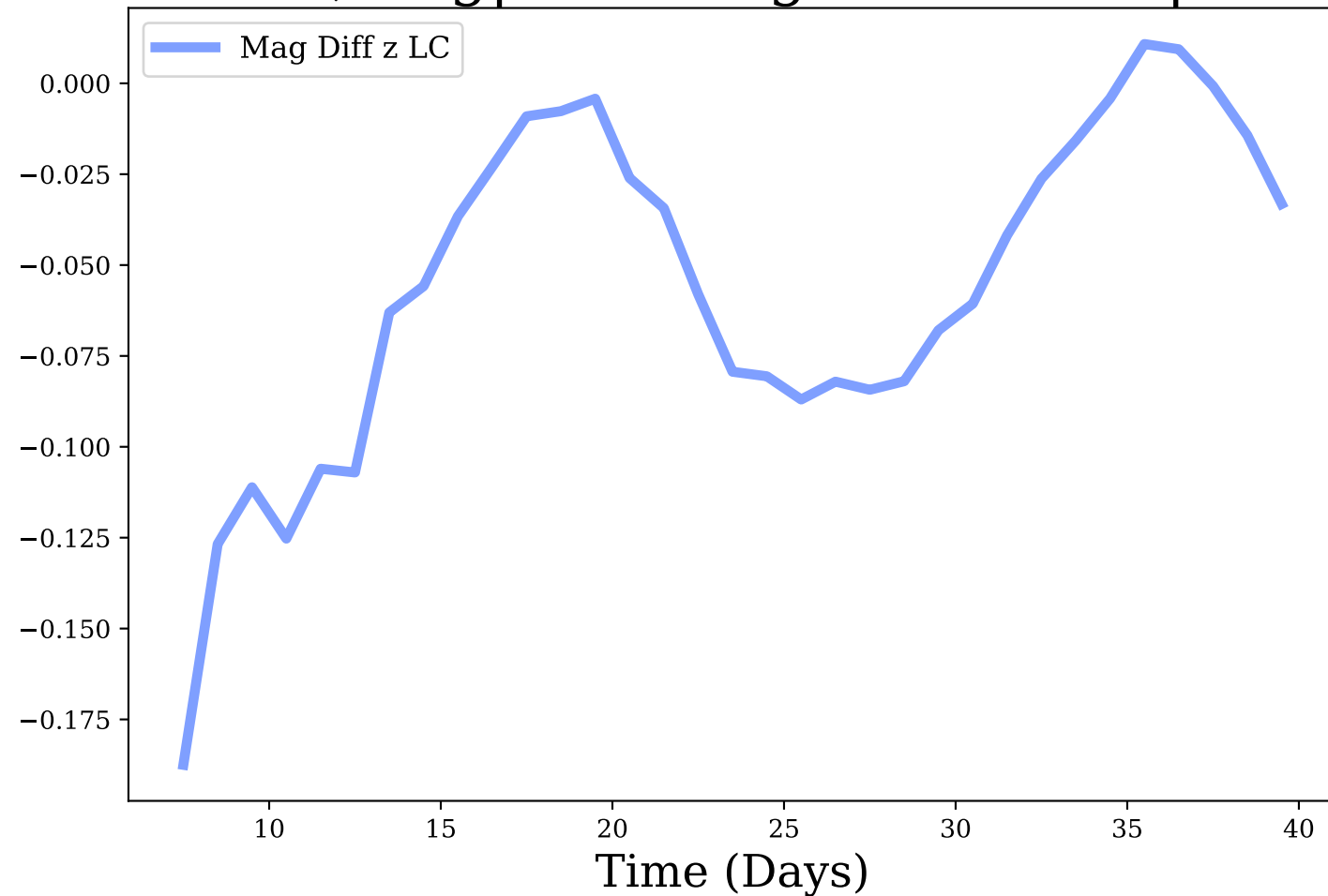
z-band, Avg|Max Mag Diff: -0.06 | 0.19
