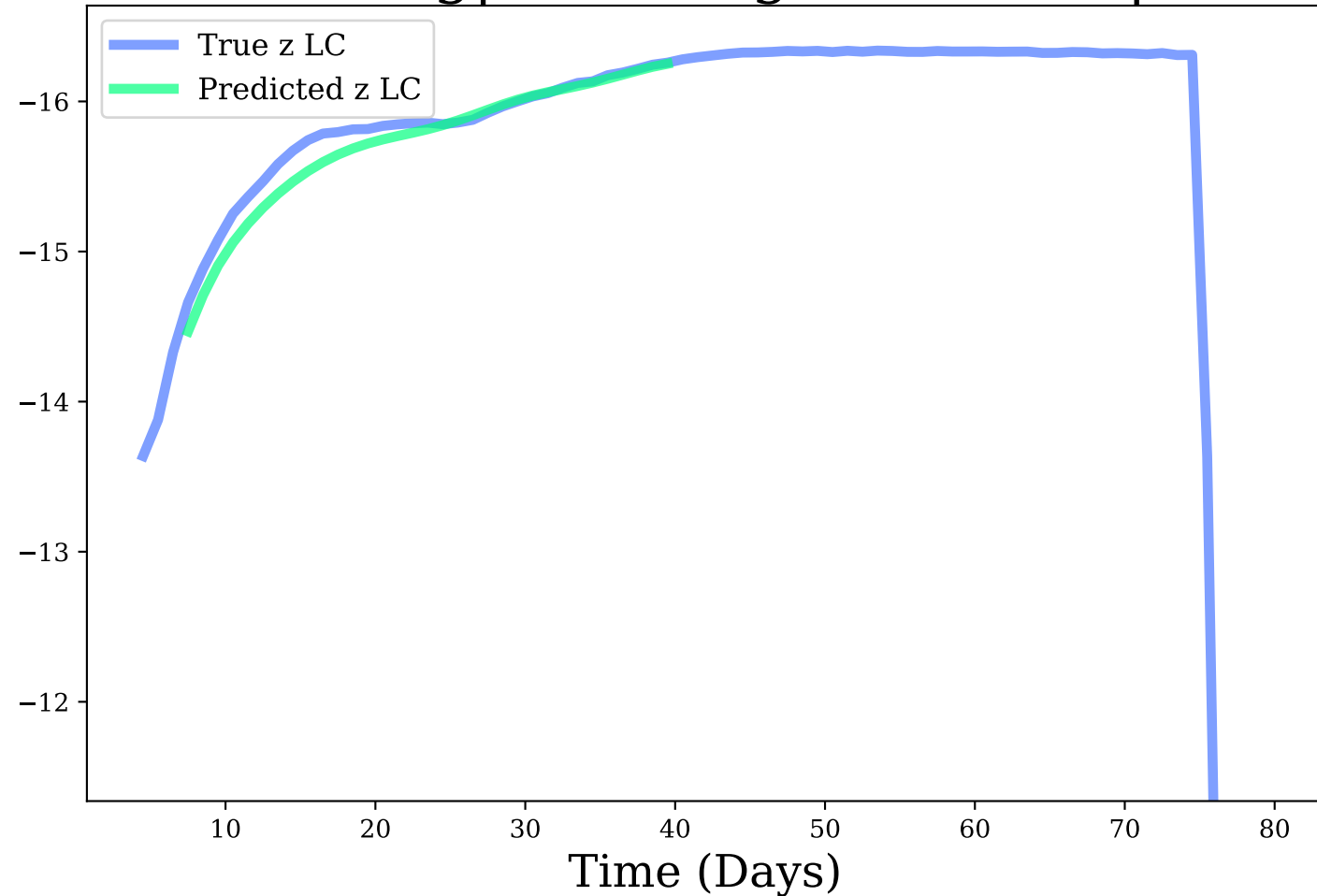
z-band, Avg|Max Mag Diff: 0.08 | 0.21
