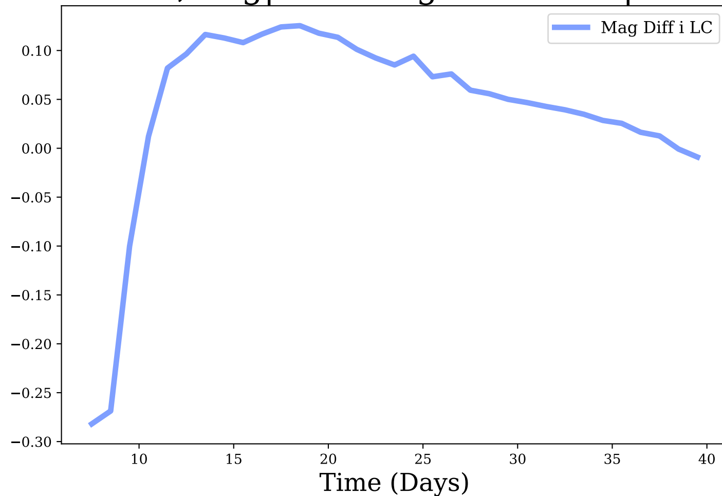
i-band, Avg|Max Mag Diff: 0.04 | 0.28
