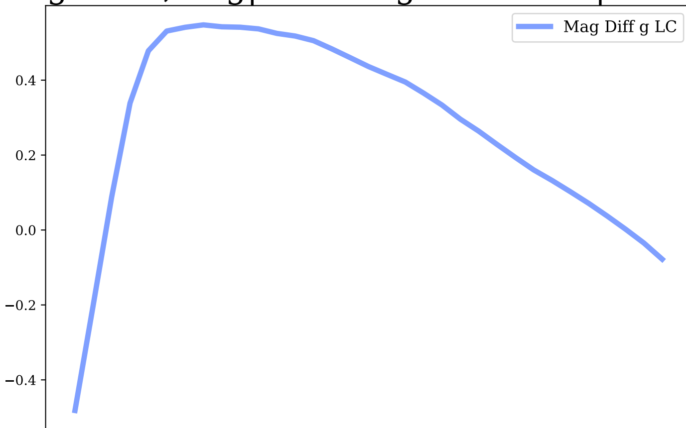
i-band, Avg|Max Mag Diff: 0.04 | 0.28
