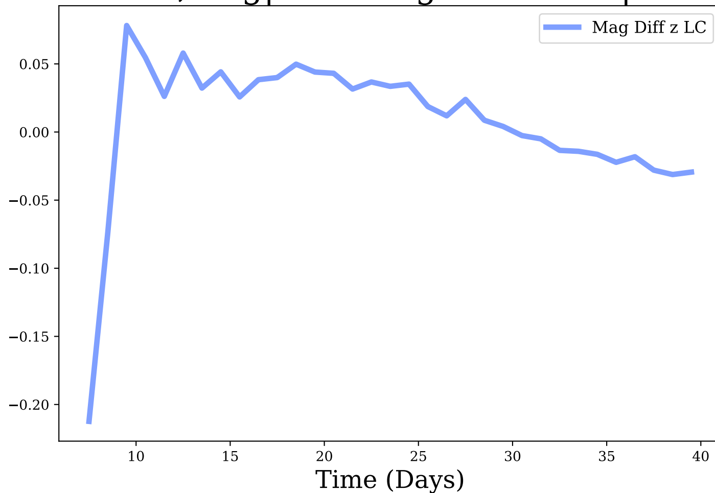
z-band, Avg|Max Mag Diff: 0.01 | 0.21
