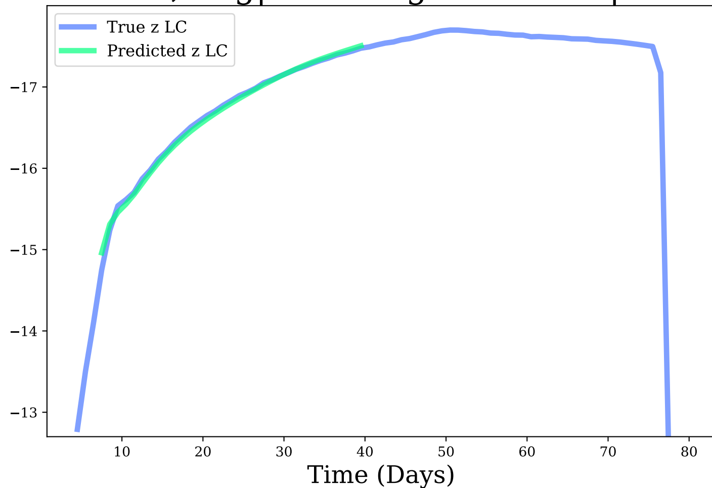
z-band, Avg|Max Mag Diff: 0.04 | 0.21
