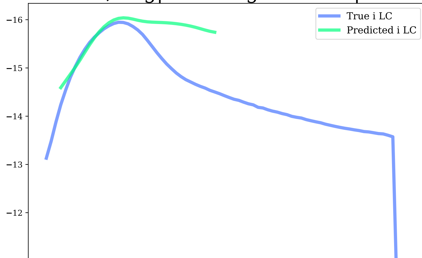
i-band, Avg|Max Mag Diff: 0.5 | 1.24
