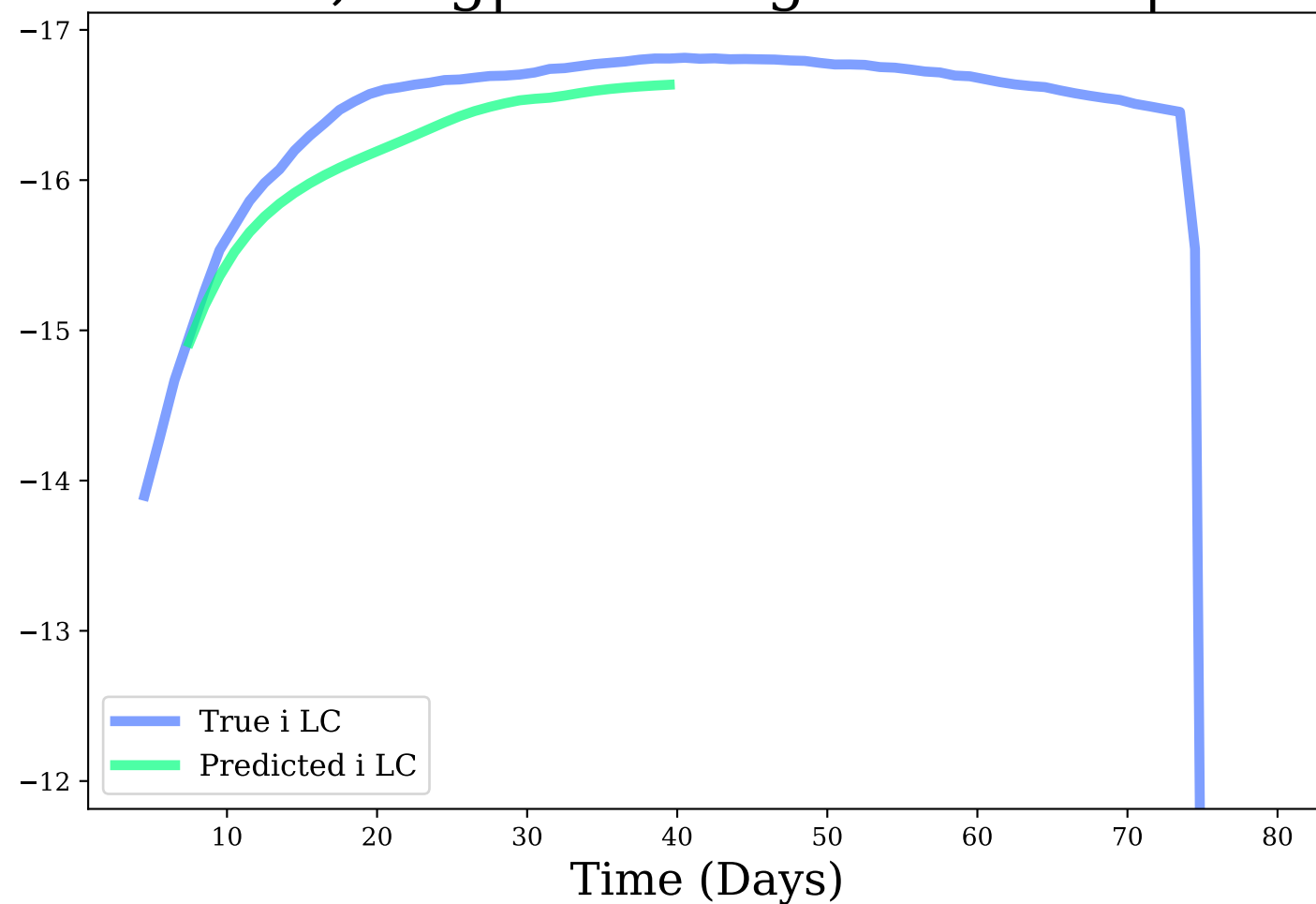
i-band, Avg|Max Mag Diff: 0.24 | 0.4
