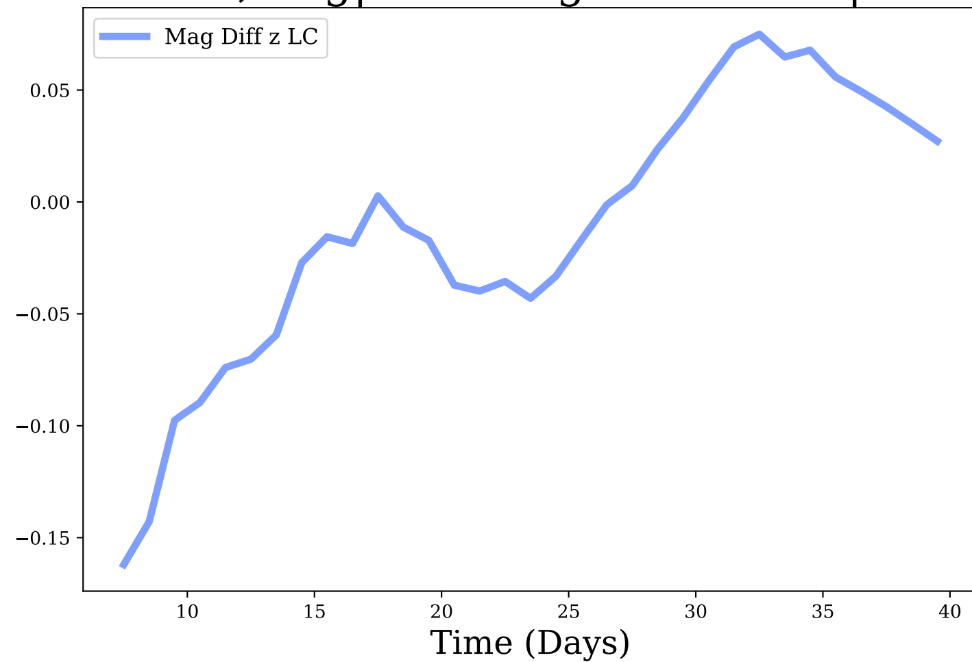
z-band, Avg|Max Mag Diff: -0.01 | 0.16
