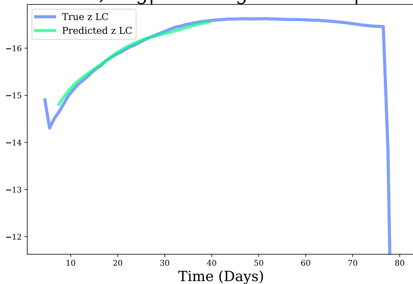
z-band, Avg|Max Mag Diff: 0.05 | 0.16
