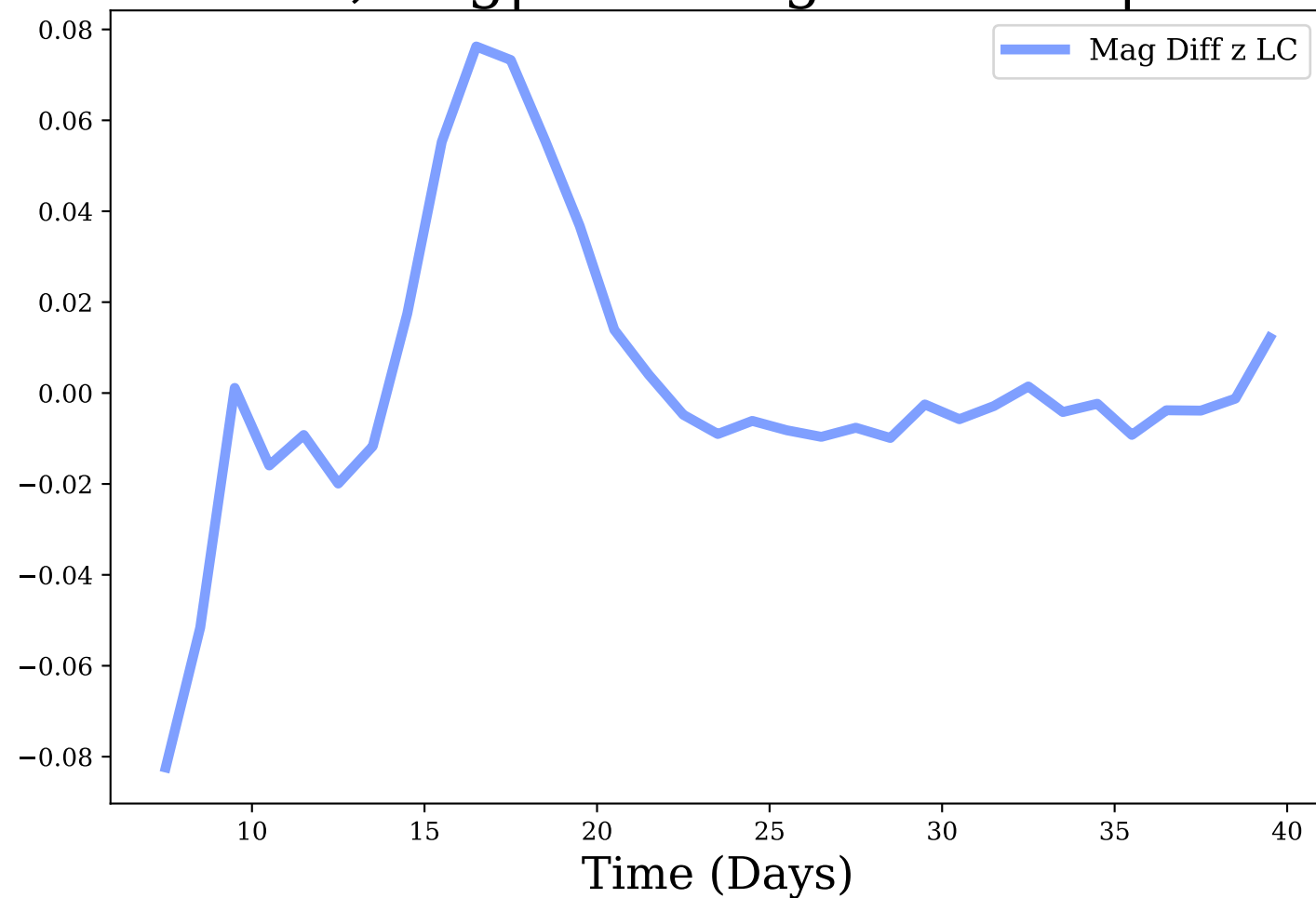
z-band, Avg|Max Mag Diff: 0.0 | 0.08
