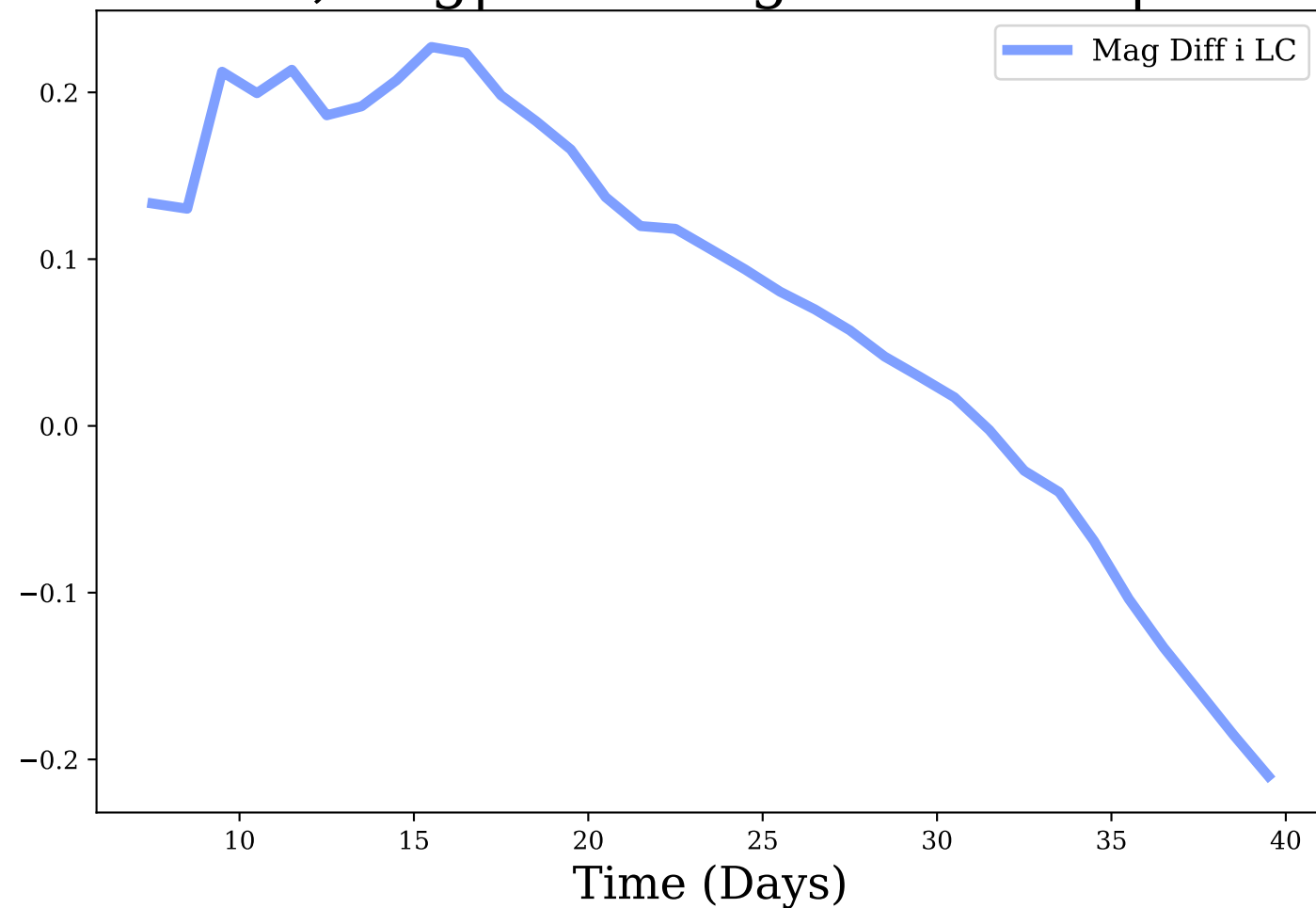
i-band, Avg|Max Mag Diff: 0.07 | 0.23
