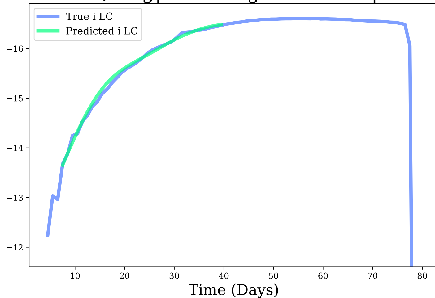
i-band, Avg|Max Mag Diff: 0.04 | 0.14
